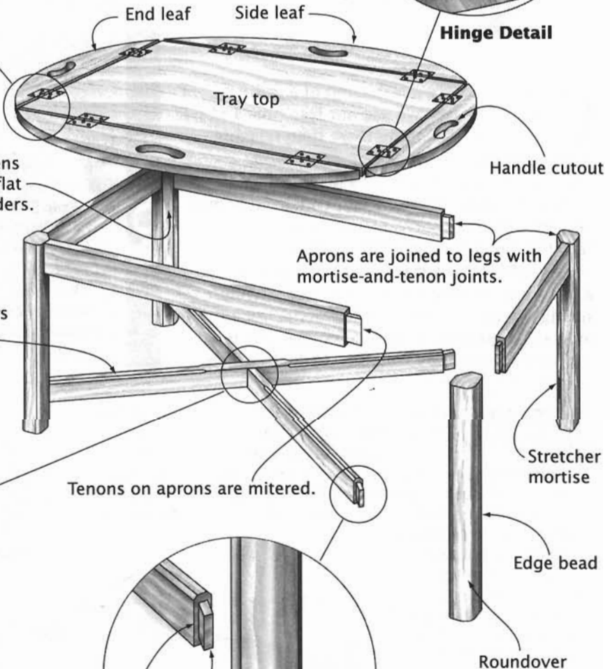
Stretcher Cross-Lap
