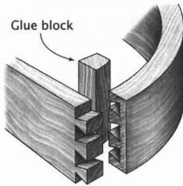
Inner Rail to Curved Apron Joinery
