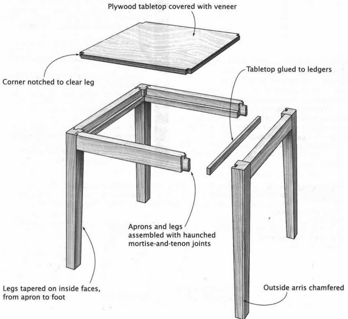
Leg-to-Apron Joinery
