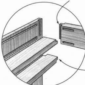
Back Rail Joinery
