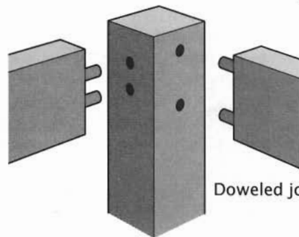
Leg-and-Apron Stand with Joinery Options
