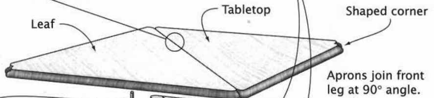
Rabbeted Rule Joint
