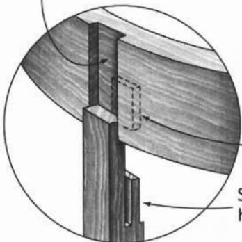
Modified Bridle Joint
