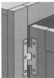
Surface-mounted hinge
