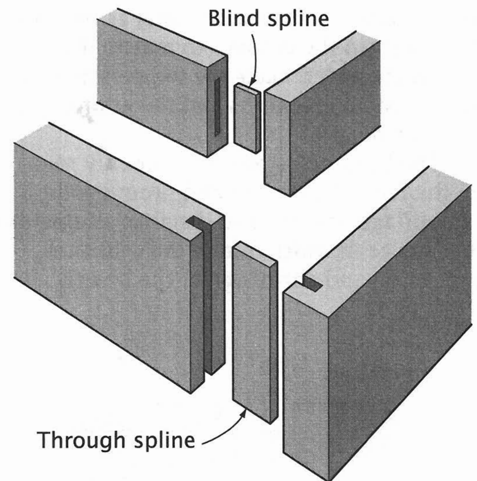
Splined Edge-to-Face Joint
