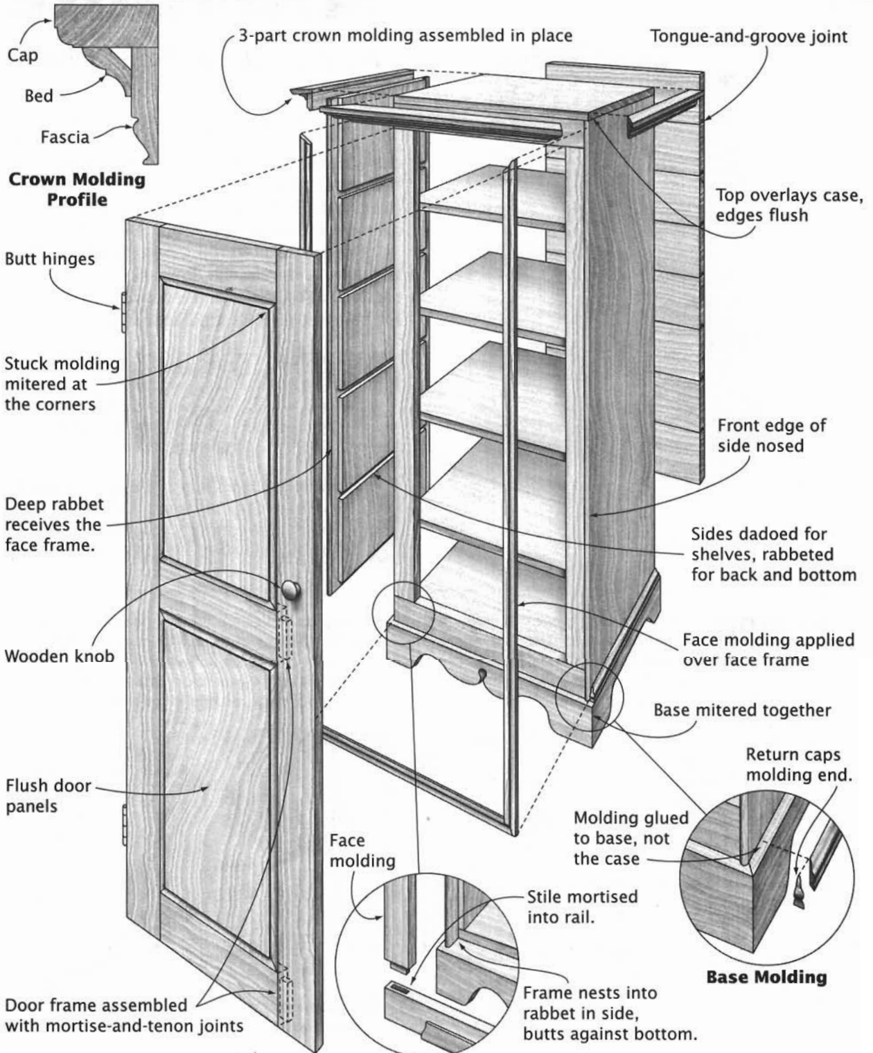
Face Frame Assembly
