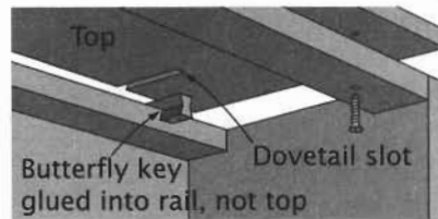
Butterfly Key
