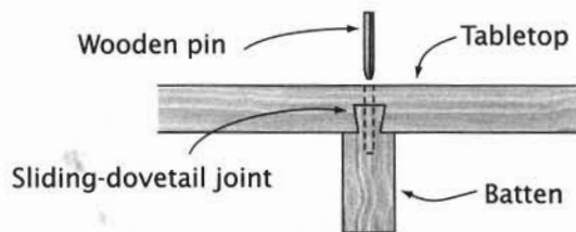
Batten-to-Tabletop Joinery
