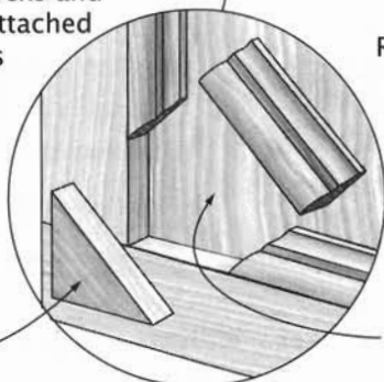
Panel Molding Installation
