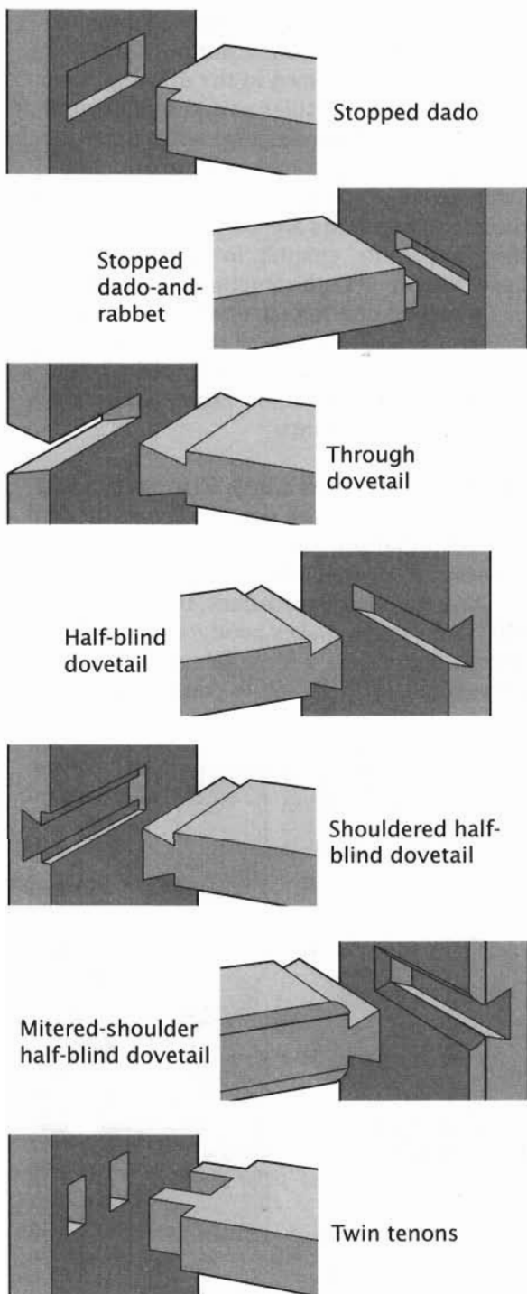
Drawer Divider Joinery
