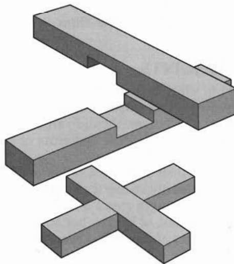
Cross-Lap
