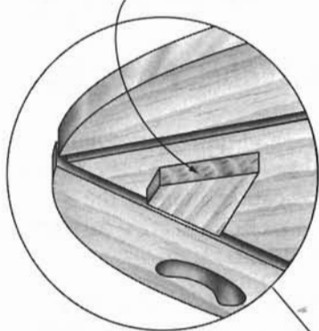
Corner Block
