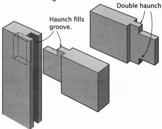
Haunched Tenon
