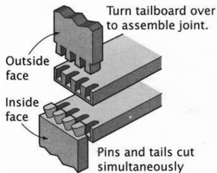
Routed
