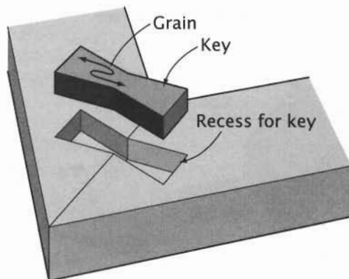
Flat Miter with Butterfly Key
