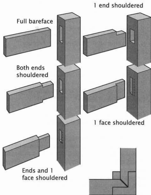
Barefaced Tenons
