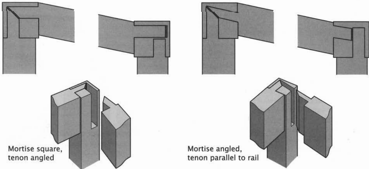
Angled Mortises and Tenons
