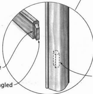
Leg-and-Stretcher Joinery
