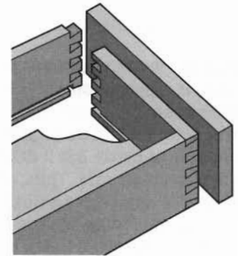
Through-dovetail joint
