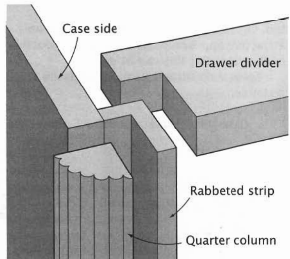
Quarter Column Construction
