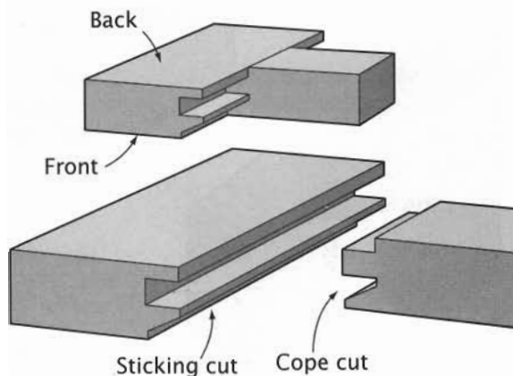
Cope-and-Stick Joint
