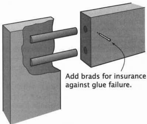
Doweled Butt
