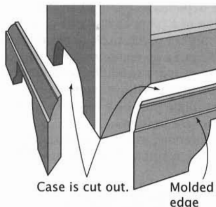
Cutout Baseboard
