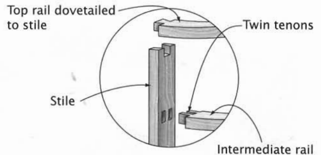
Rail-and-Stile Joinery
