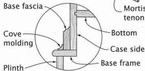
Base Molding Assembly
