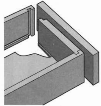
Dado-and-rabbet joint
