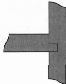
Dado-and-rabbit joint
