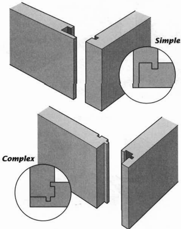
Lock Joints
