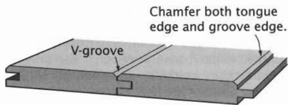
Tongue-and-Groove Joint
