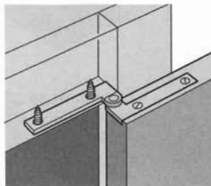
Knife hinge
