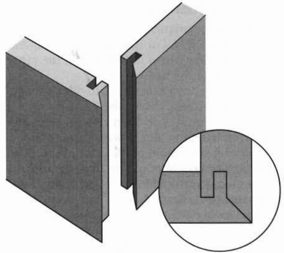
Lock Miter Joint
