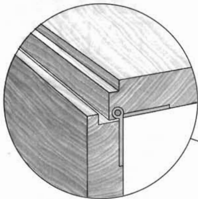
Rabbeted Rule Joint
