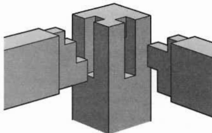
Mortise-and-interlocked-tenon joint
