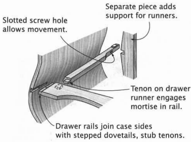
Drawer Runner Construction
