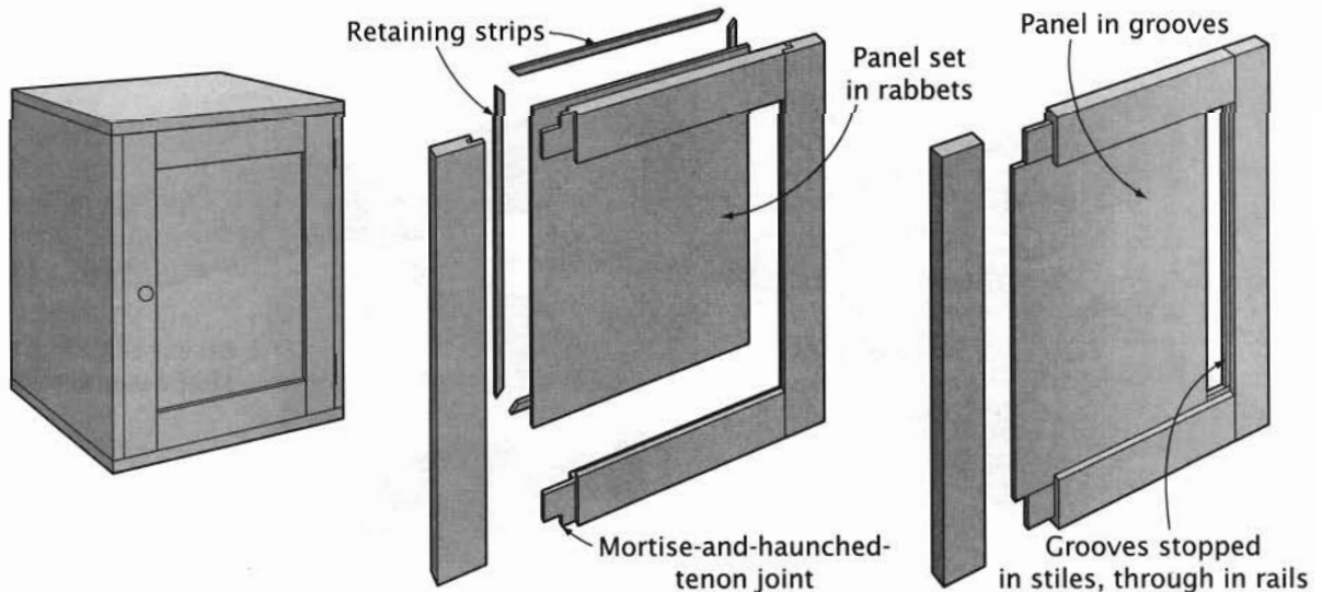
Rabbeted Construction
