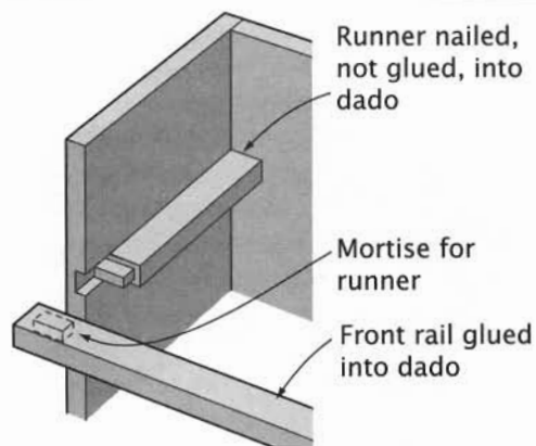
Rail and Runner
