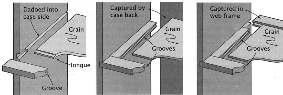
Dust Panel
