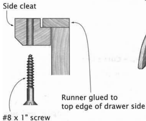
Drawer Runner
