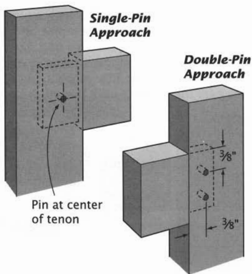
Pegged Mortise-and-Tenon
