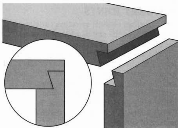
Dovetailed Rabbet
