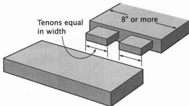
Double Mortise-and-Tenon
