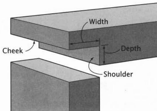
Single-Rabbet Joint
