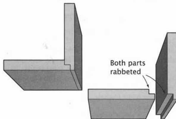
Double-Rabbet Joint
