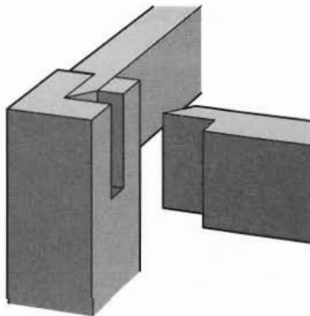
Mortise-and-barefaced-tenon joint
