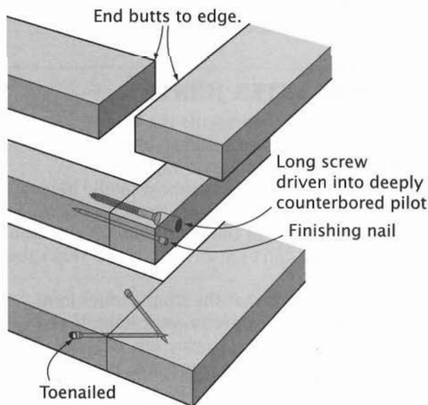
Butt Joint
