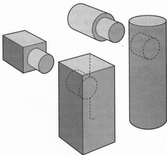
Round Mortise-and-Tenon
