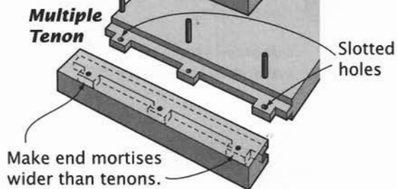
Mortise-and-Tenon Breadboard
