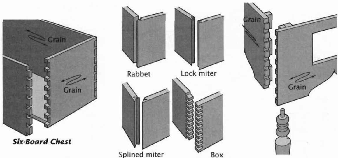
Alternate joints
