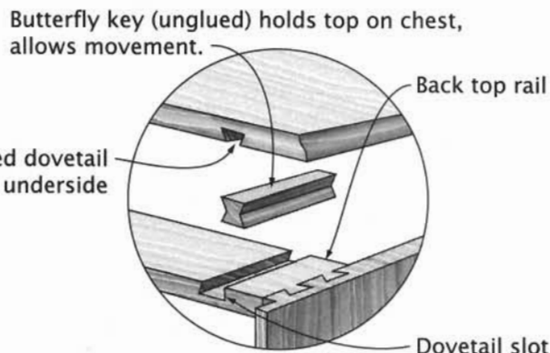
Top-to-Case Joinery
