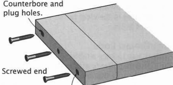
Butt Joint with Screws
