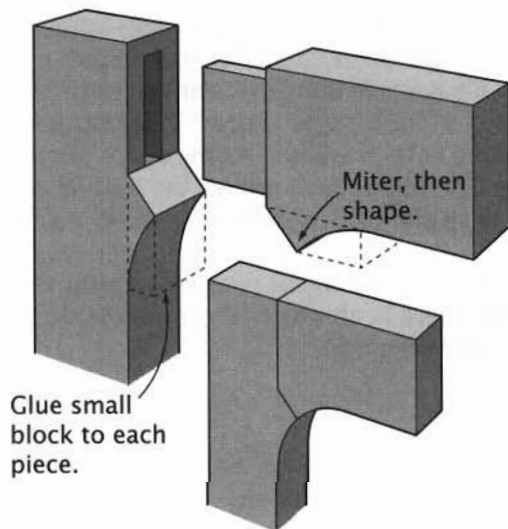
Mortise-and-Tenon with Mitered Shoulders
