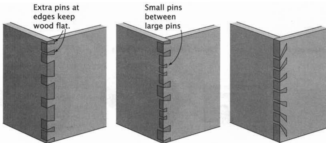
Varied Spacing of Pins and Tails
