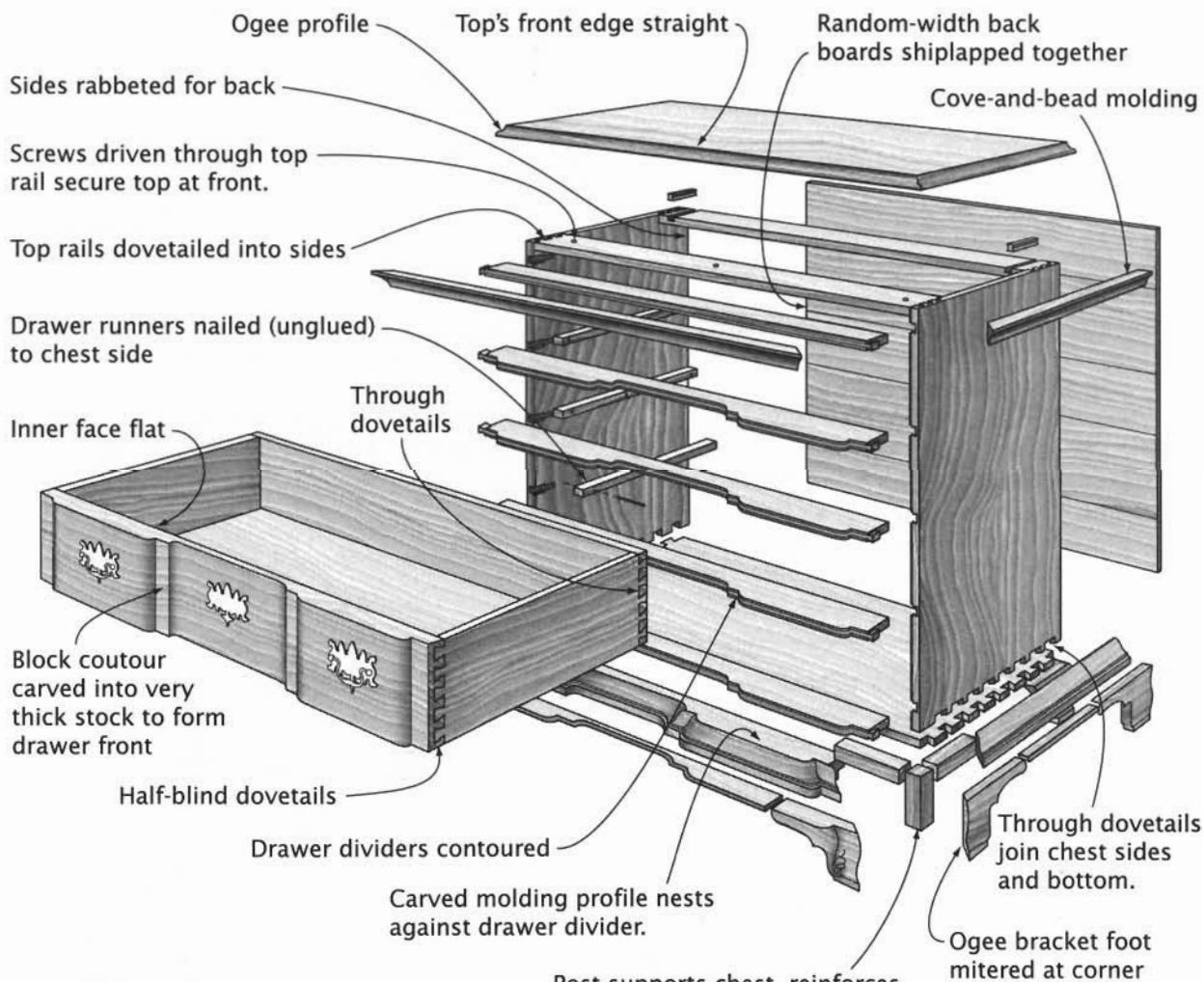
Drawer Divider-to-Case Joinery
