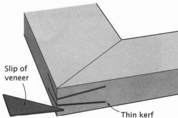
Flat Miter with Feather Keys
