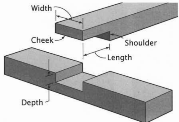
Lap Joint Particulars
