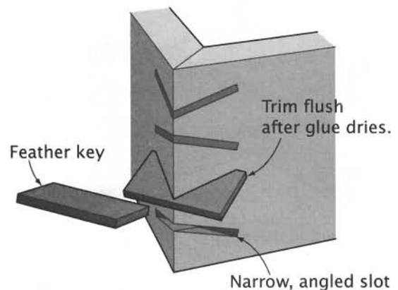
End Miter with Feather Keys
