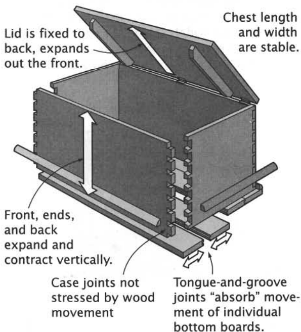
Chest Construction
