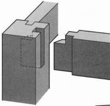
Mortise-and-haunched-tenon joint
