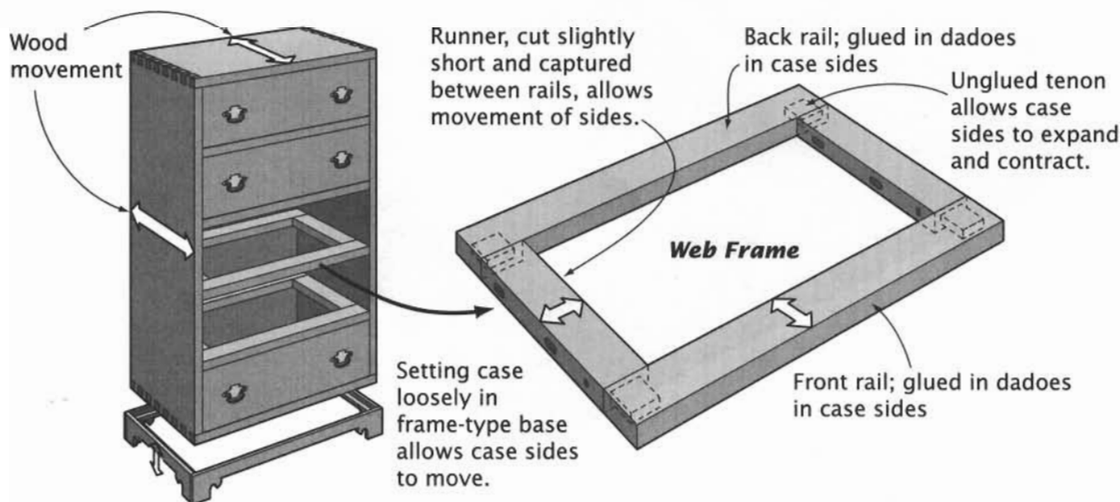
Case Construction
