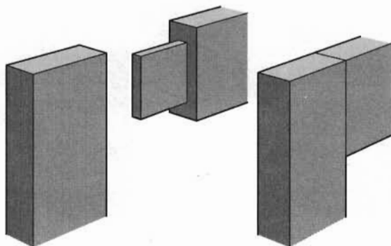
Blind Mortise-and-Tenon
