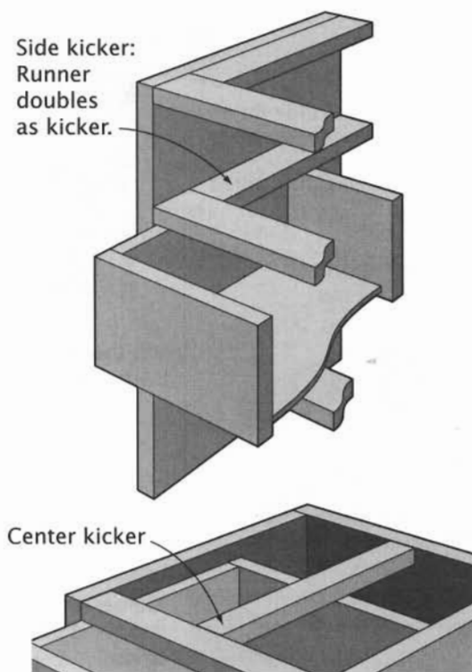
Kickers
