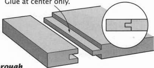
Through Tongue-and-Groove
