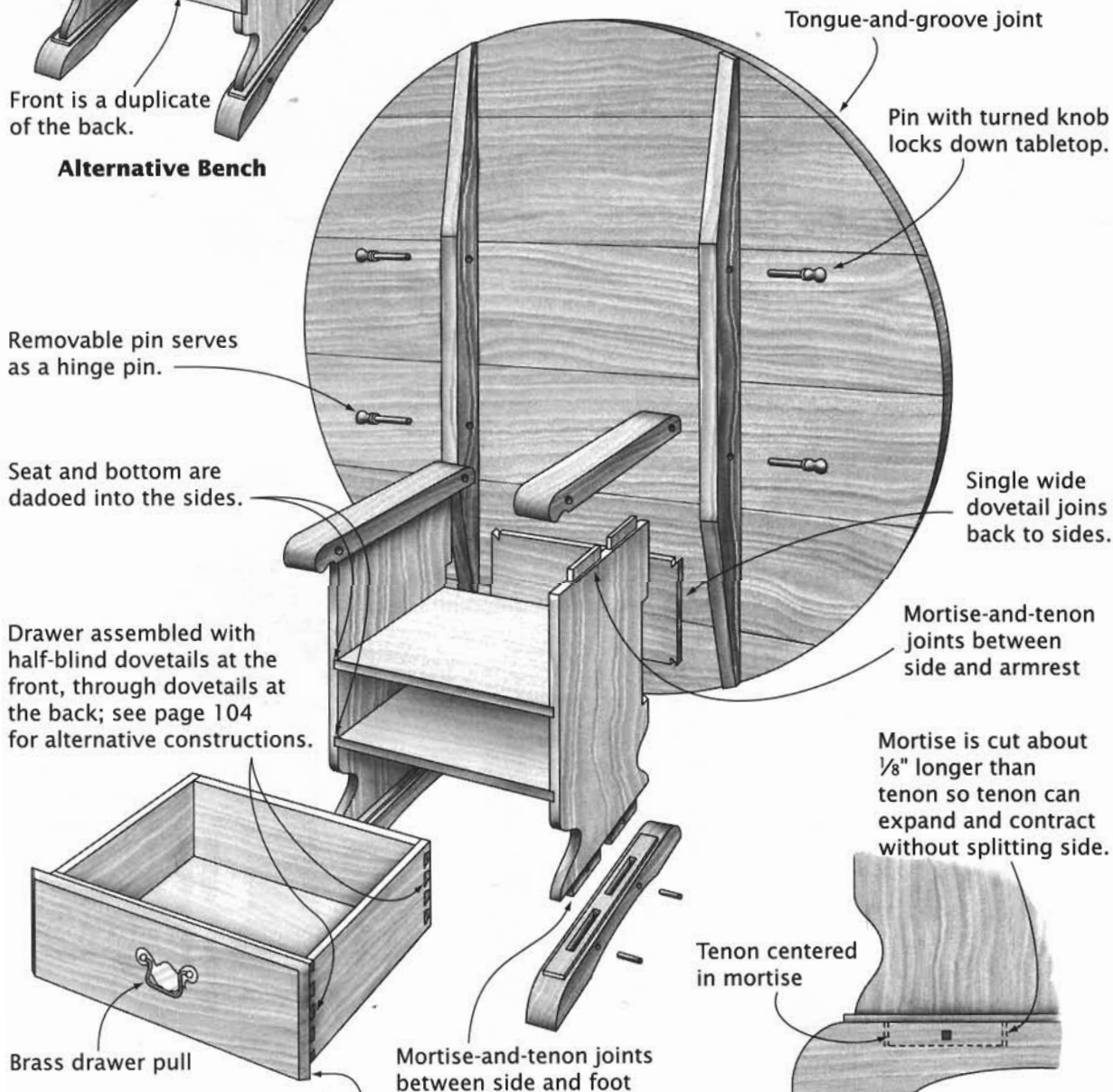
Side-to-Foot Joinery
