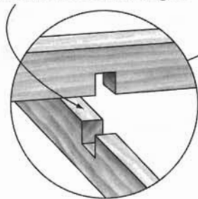
Stretcher Cross-Lap
