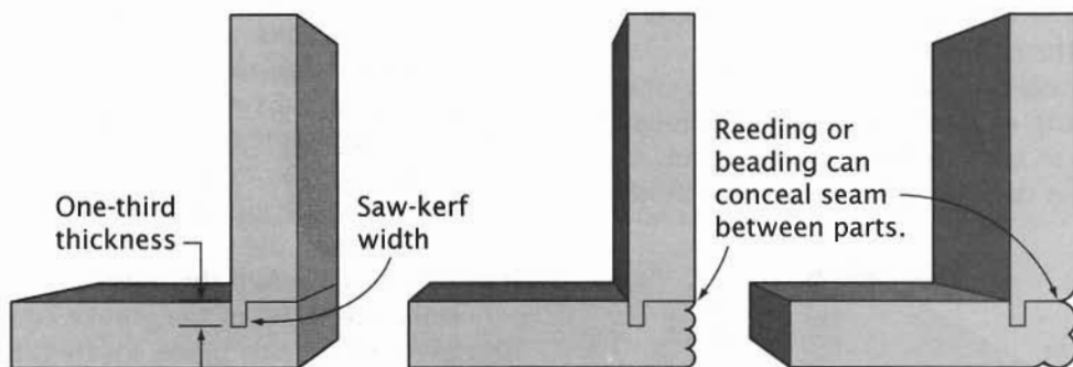
Rabbet-and-Groove Joint
