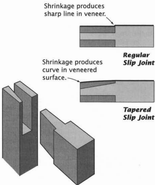
Tapered Slip Joint
