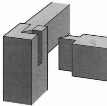
Full-height mortise-and-tenon joint
