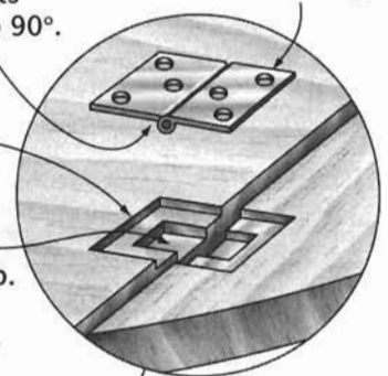
Hinge Detail
