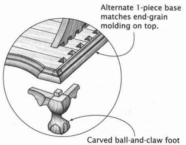
Alternative Construction
