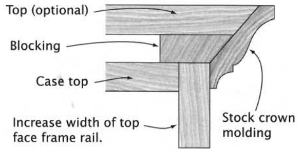
Optional Crown Molding
