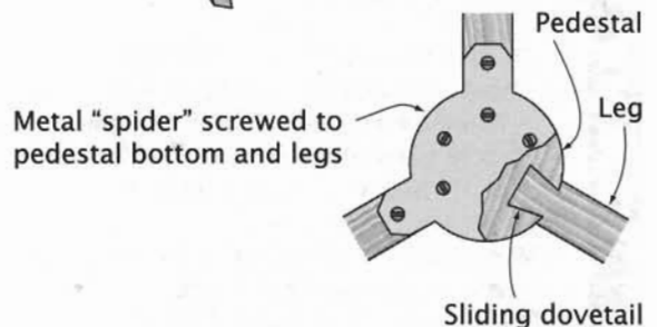
Leg-to-Pedestal Joinery
