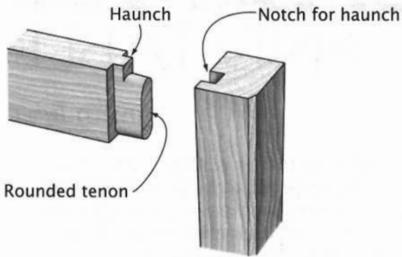
Leg-to-Apron Joinery
