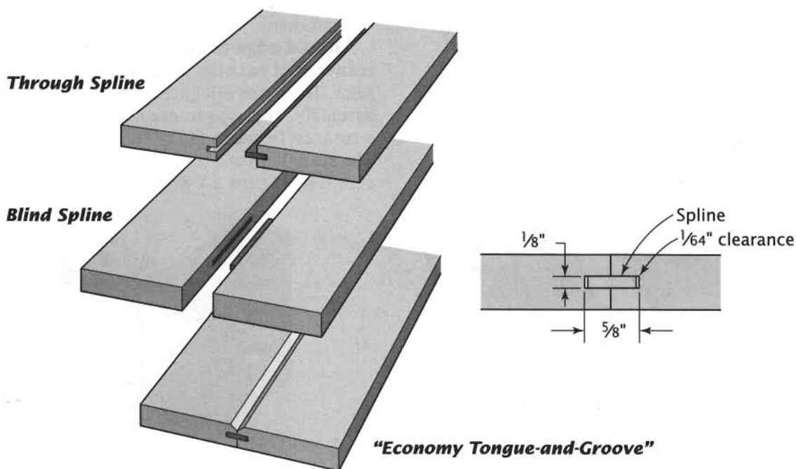
Splined Edge-to-Edge Joints
