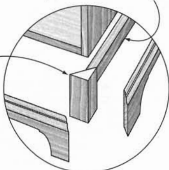
Base Joinery
