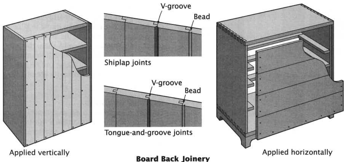
Board Back Joinery
