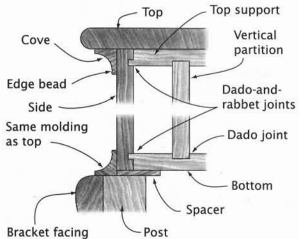
Case Joinery
