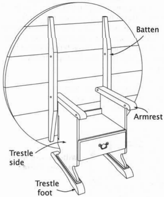
Settle Chair-Table
