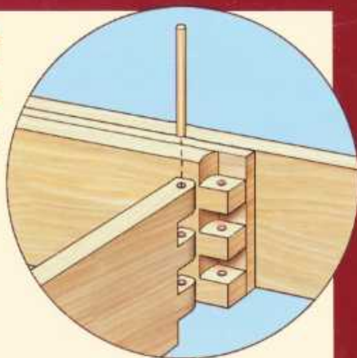
Knuckle Joint
