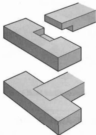
Pocket Lap
