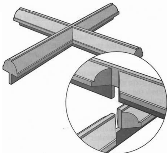
Glazing-Bar Cross-Lap
