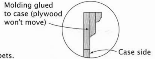
Cornice Molding Assembly
