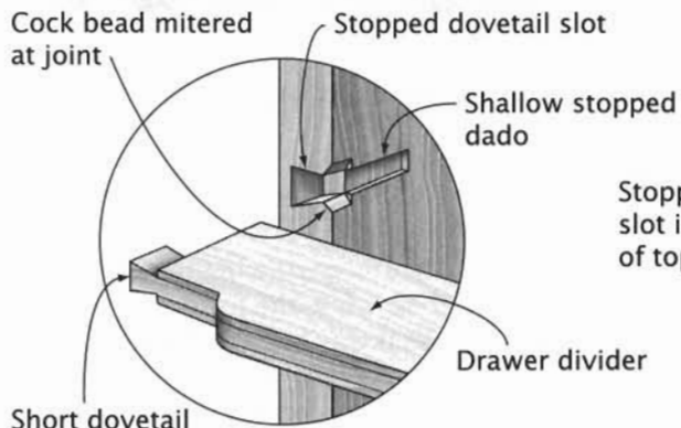
Drawer Divider-to-Case Joinery
