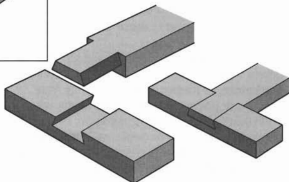
Dovetail-Keyed Half-Lap
