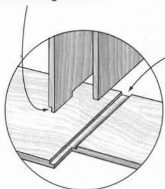
Partition Joinery
