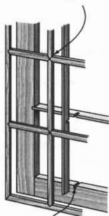
Slot for spine Muntin Assembly
