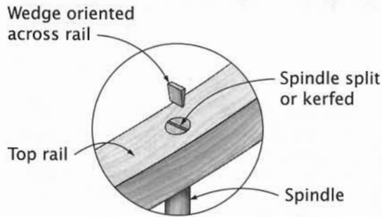
Wedged Spindle
