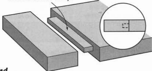
Blind Tongue-and-Groove
