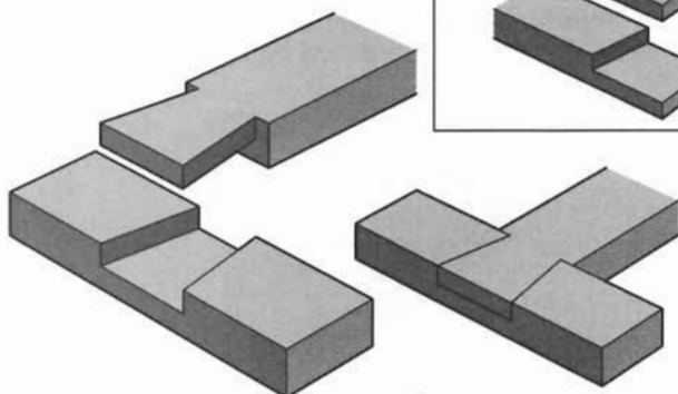
Dovetailed Half-Lap
