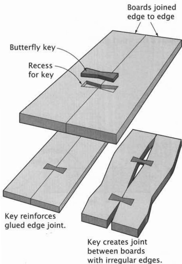
Butterfly Key
