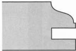
Roman ogee
