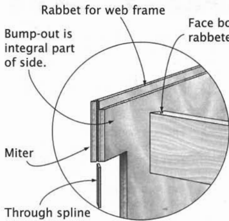
Overhang Construction
