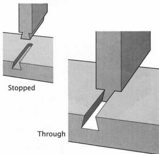
Sliding Dovetail
