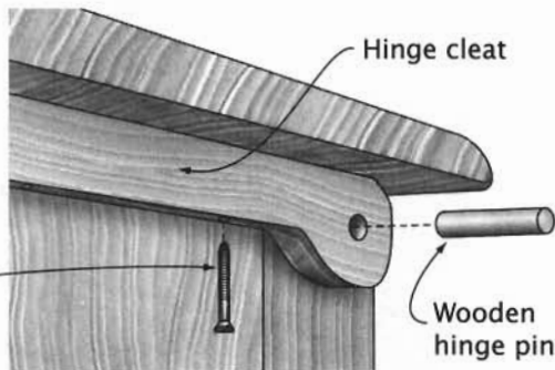
Hinge Detail
