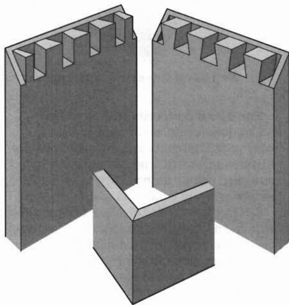
Full-Blind Dovetails
