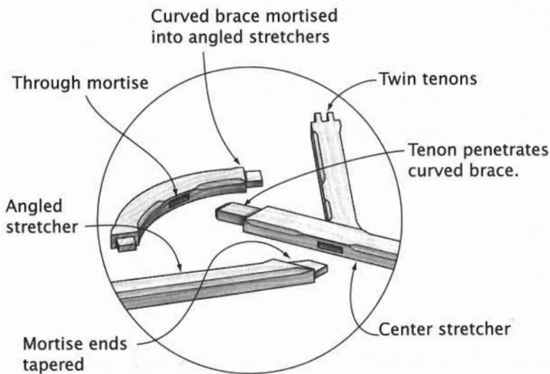
Hayrake Stretcher Joinery
