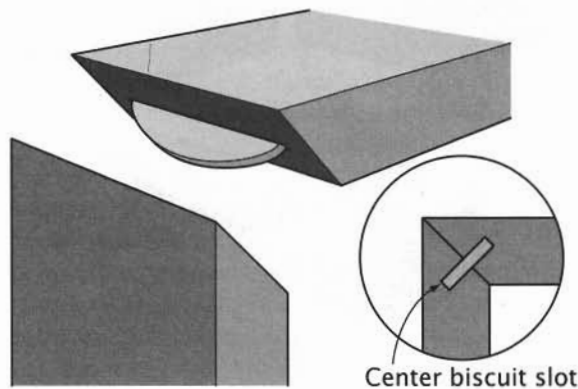
Biscuited End Miter
