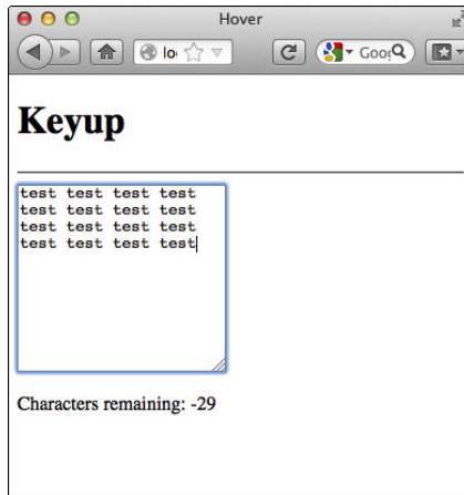
Figure 4-9: Entering characters past the limit.
