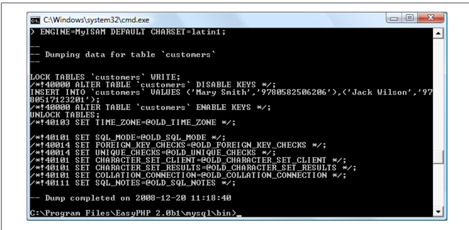
Figure 9-4. Dumping the publications database to the screen
