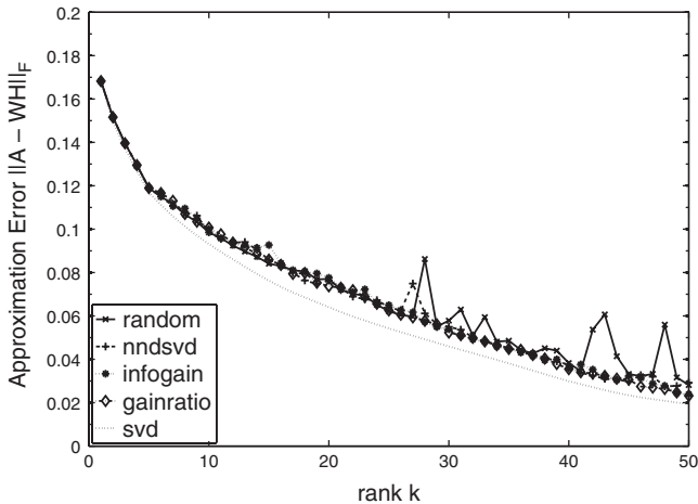
Figure 4.4 Approximation error for different initialization strategies and varying rank k using the ALS algorithm ( maxiter = 30 ).
