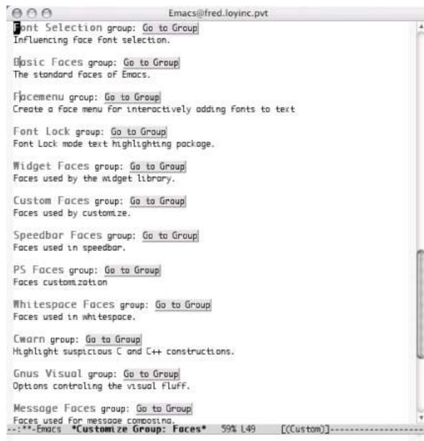
Figure 10-10. Font face groups available in Custom (Mac OS X)
