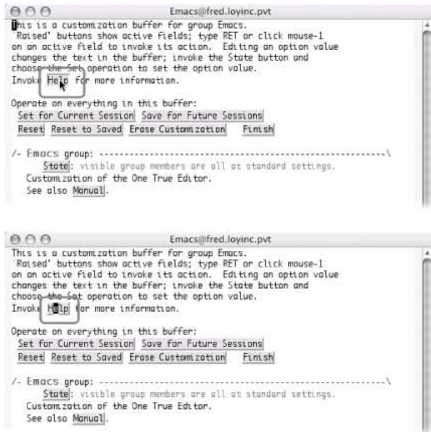
Figure 10-1. Custom button activation using the mouse cursor (top) and the keyboard cursor (bottom) (Mac OS X)
