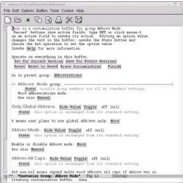
The Abbrev Mode group.
