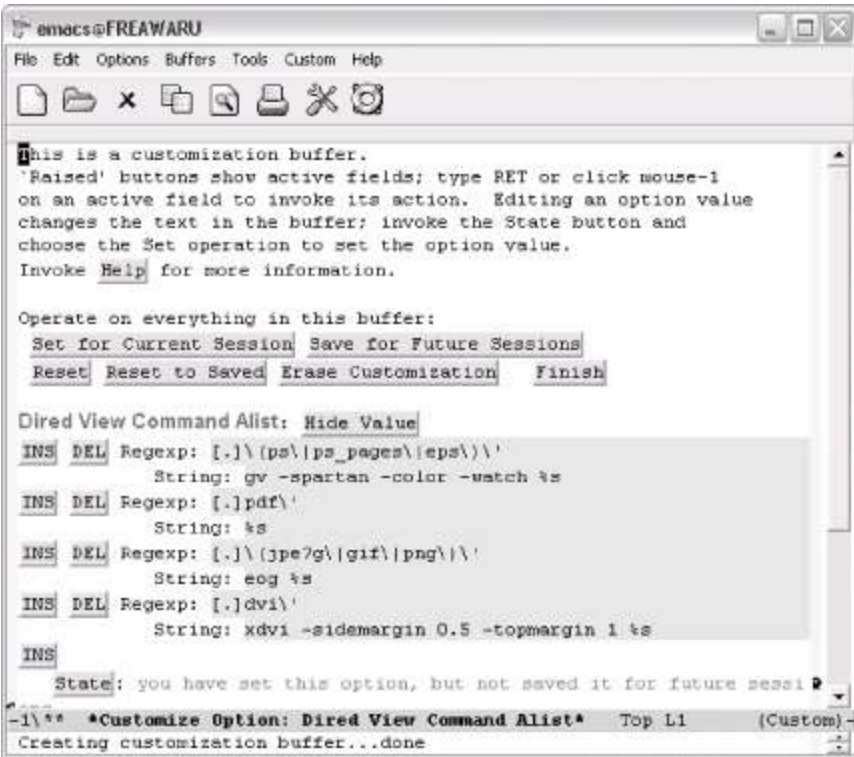
Editing a list entry in Custom (Windows).
