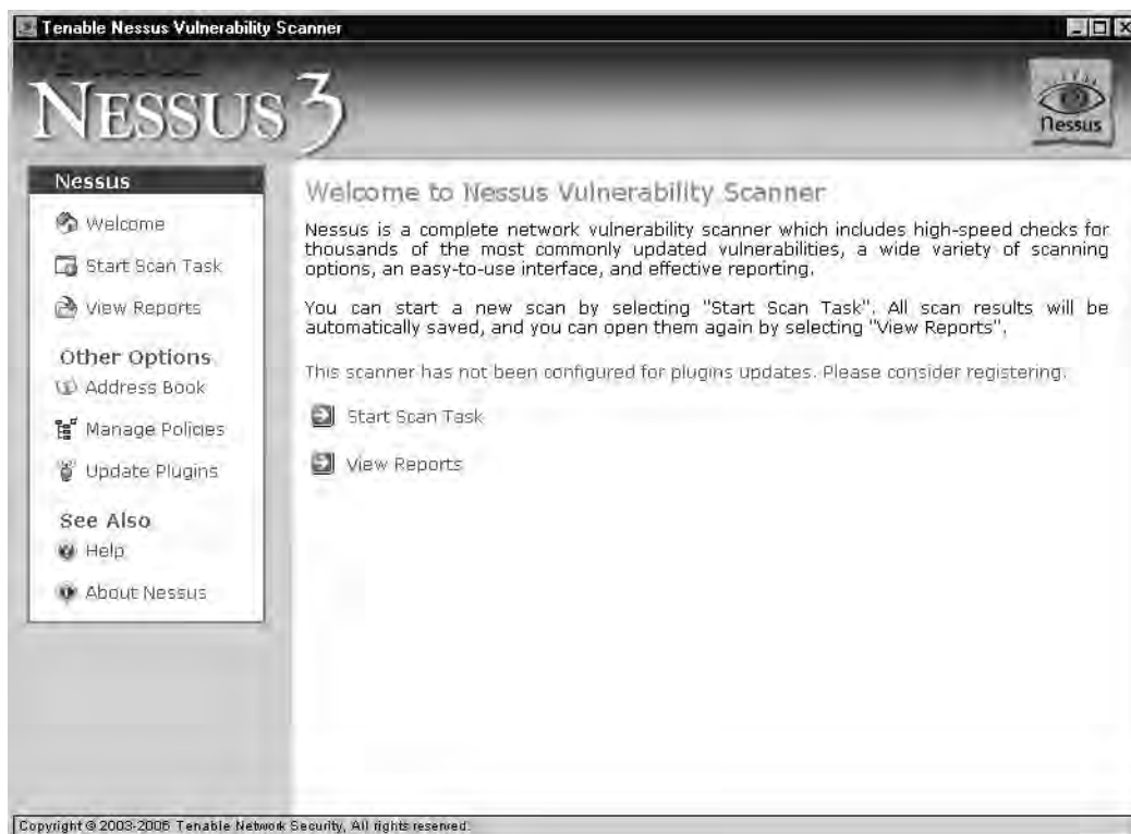
Figure 6.13 Windows Nessus
