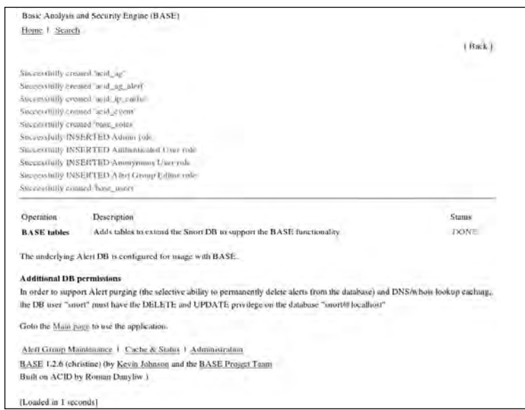
Figure 4.16 BASE Success
