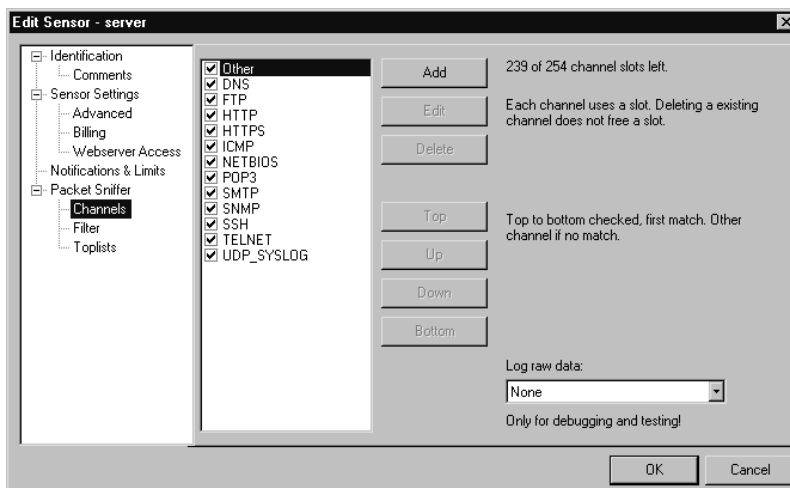
Figure 7.8 Edit Sensor
