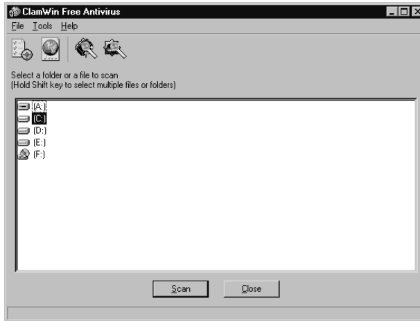
Figure 3.22 ClamWin
