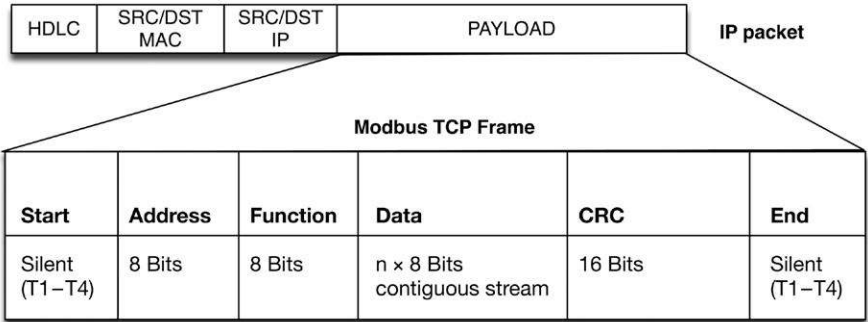
FIGURE 4.4 Modbus Frame (Modbus TCP).
