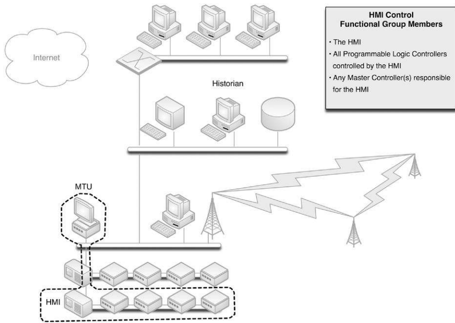
FIGURE 7.2 A Functional Group Based on an HMI.
