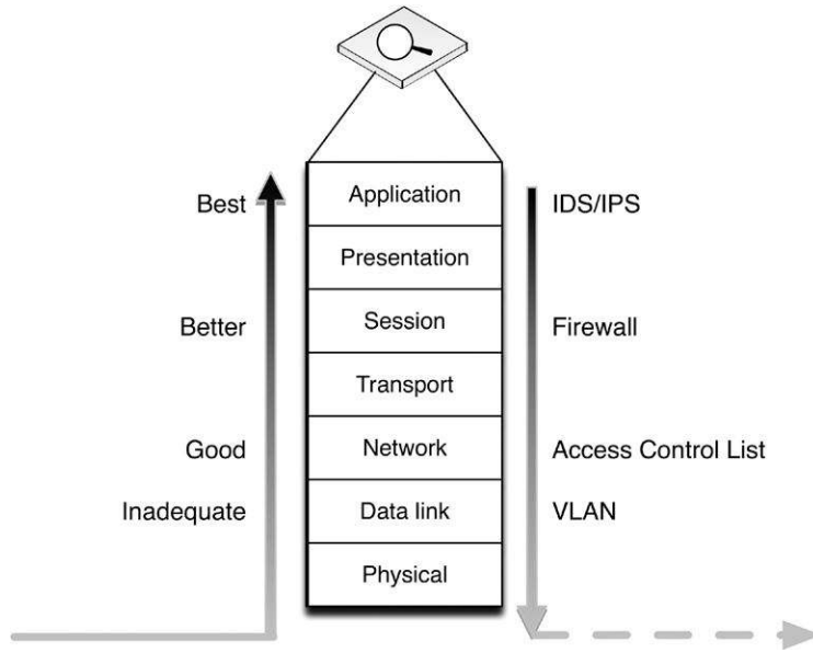
FIGURE 7.14 Relative Capabilities of Common Security Devices.
