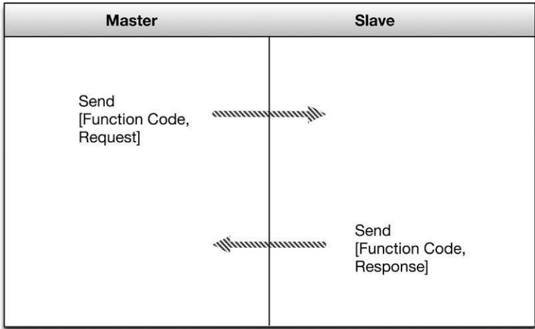
FIGURE 4.1 Modbus Protocol Operation.
