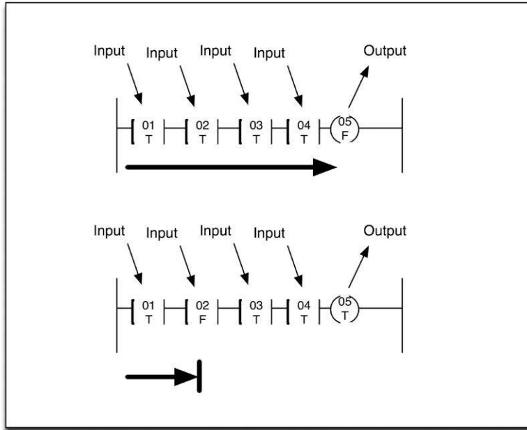
FIGURE 5.2 Example of Simple Ladder Logic, with Both Complete and Incomplete Conditions.
