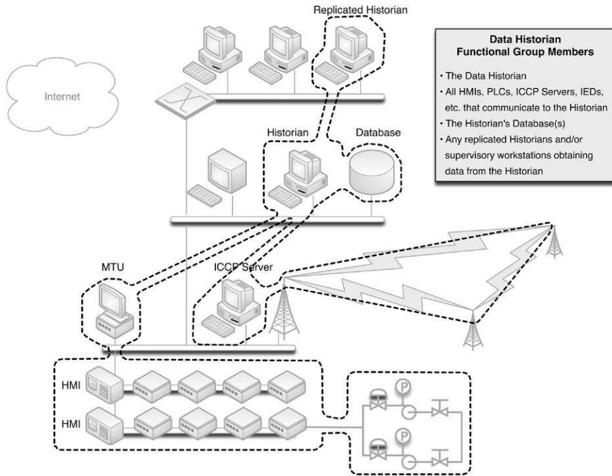
FIGURE 7.4 A Functional Group Based on Historization.
