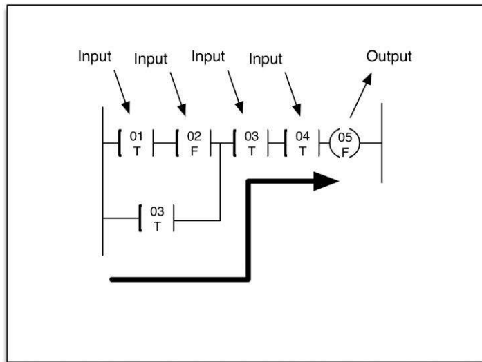
FIGURE 5.3 Example of Simple Ladder Logic, Containing an “or” Condition.
