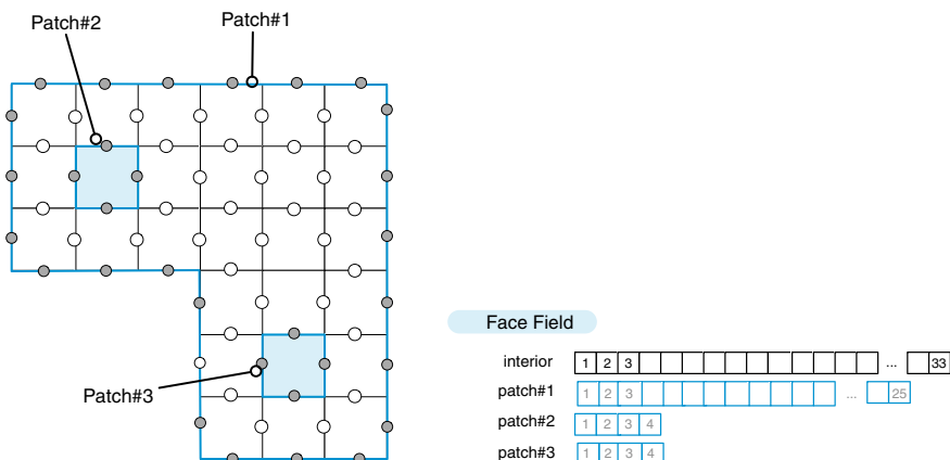
Fig. 4.15 Face field
