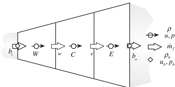
Fig. 16.6 Diverging nozzle
