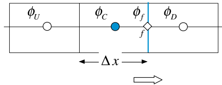
Fig. 12.22 A one dimensional uniform grid
