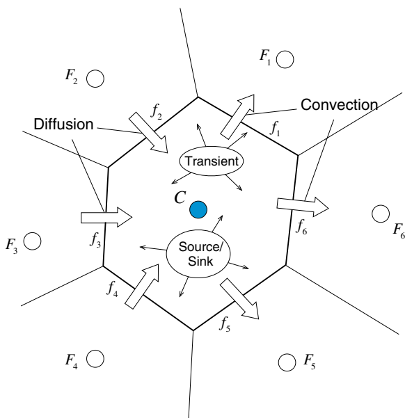
Fig. 15.15 Element C in a general unstructured grid system
