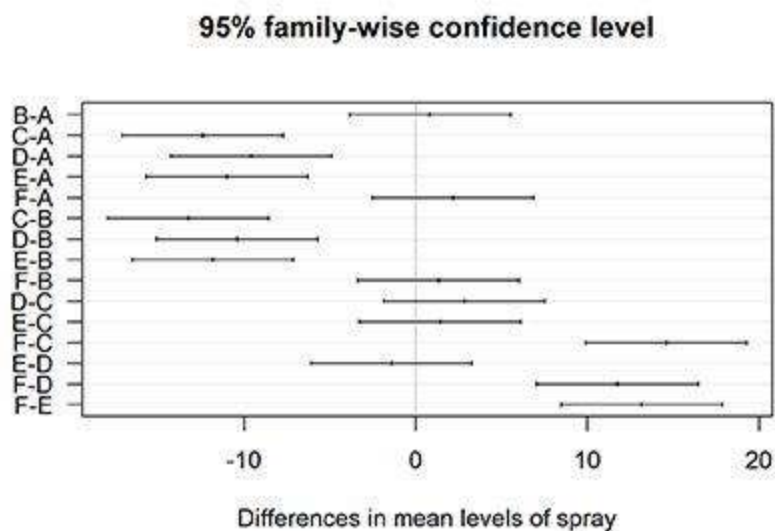
Figure 15-4: Plotting the results of Tukey's HSD test.
