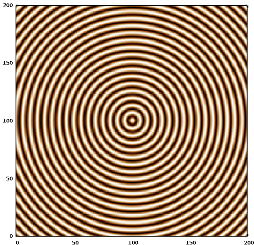
Figure of a two dimensional sin function.
