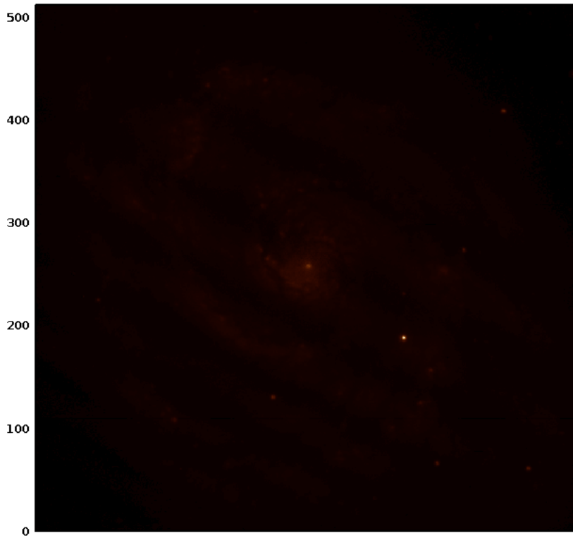
Figure of the raw image m51_raw.fits shown with progressively greater contrast using the imag command.
