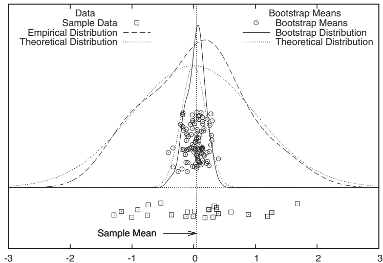
FIGURE 12-4. The bootstrap. The points in the original sample are shown at the bottom; the means calculated from the bootstrap samples are shown above. Also displayed are the original distribution and the distribution of the sample means, both using the theoretical result and a kernel density estimate from the corresponding samples.
