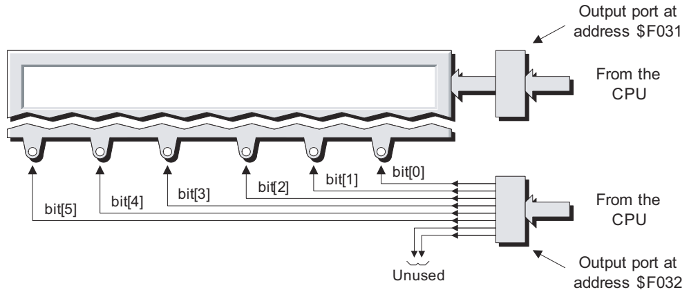
Figure L2-19. The calculator's six LEDs.
