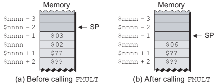
Figure L3-19. Example stack contents before and after calling the FMULT subroutine.
