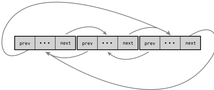
Figure 6.4 A circular doubly linked list.
