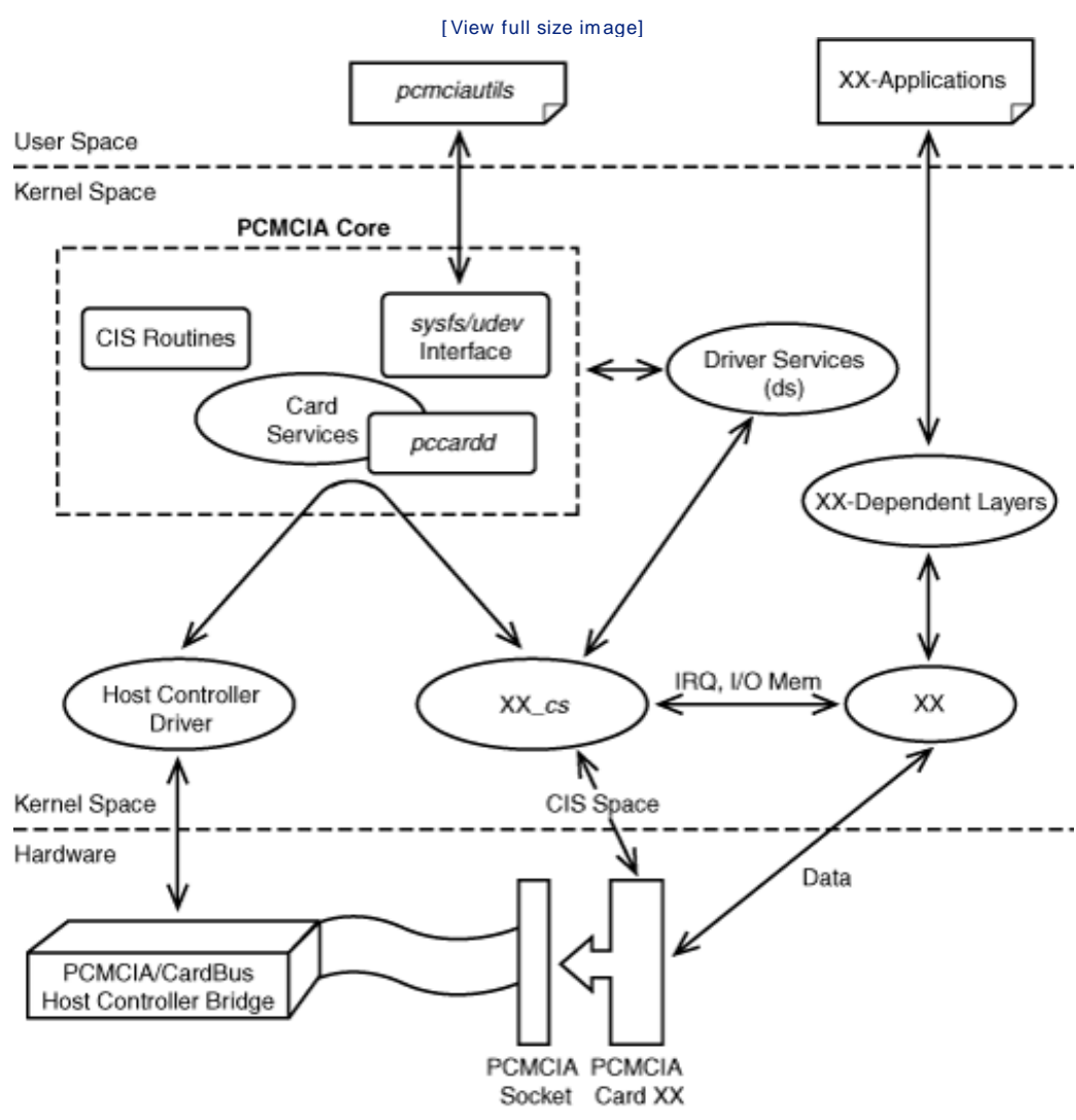
Figure 9.3. The Linux-PCMCIA subsystem.
