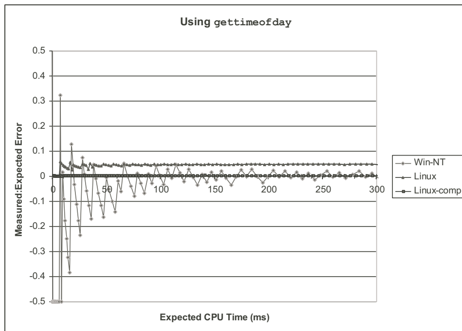
Figure 9.22: Experimental Validation of K -Best Measurement Scheme Using gettimeofday Function. Linux implements this function using cycle counters and hence achieves the same accuracy as our own timing routines. Windows-NT implements this function using interval counting, and hence the accuracy is low, especially for small duration measurements.
