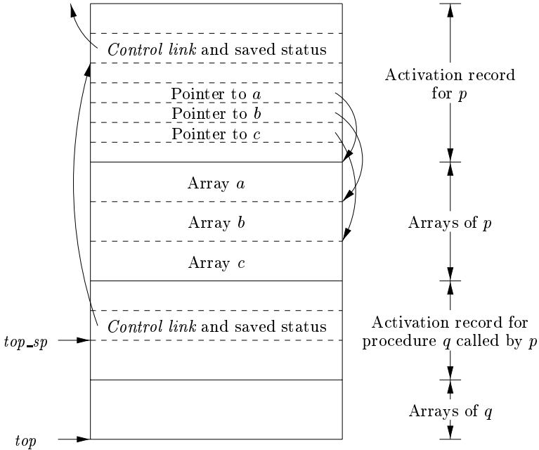
Figure 7.8 Access to dynamically allocated arrays
