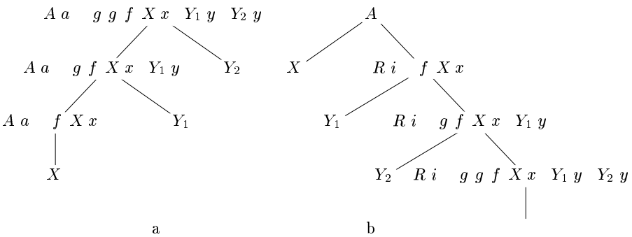
Figure 5.23 Eliminating left recursion from a post-x SDT
