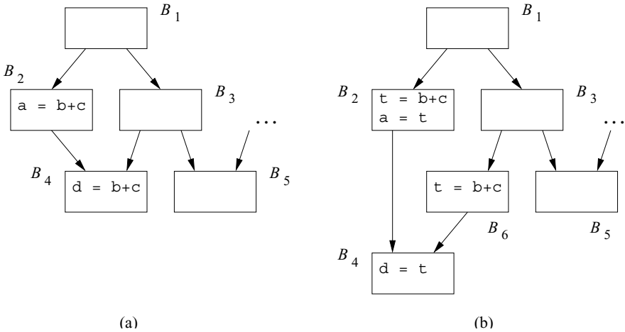
Figure 9 31 B_3 - B_4 is a critical edge
