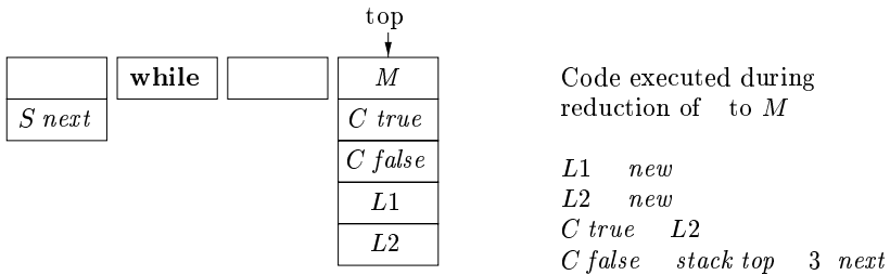
Figure 5.36 LR parsing stack after reduction of M
