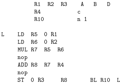
Figure 10 17 Locally scheduled code for Example 10 12
