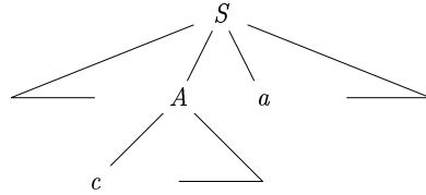
Figure 4.15 Terminal c is in FIRST(A) and a is in FOLLOW(A)
