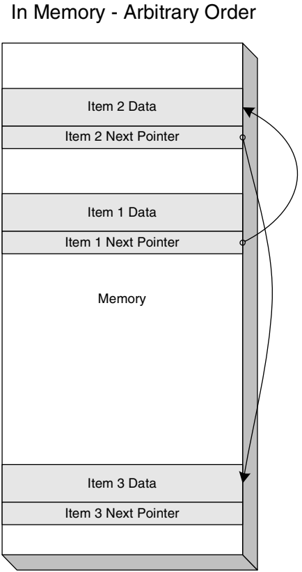
Figure C.2 Logical and in-memory arrangement of a singly linked list.
