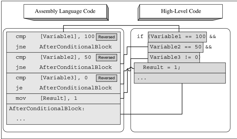
Figure A.10 High-level/low-level view of a compound conditional statement with three conditions combined using the AND operator.
