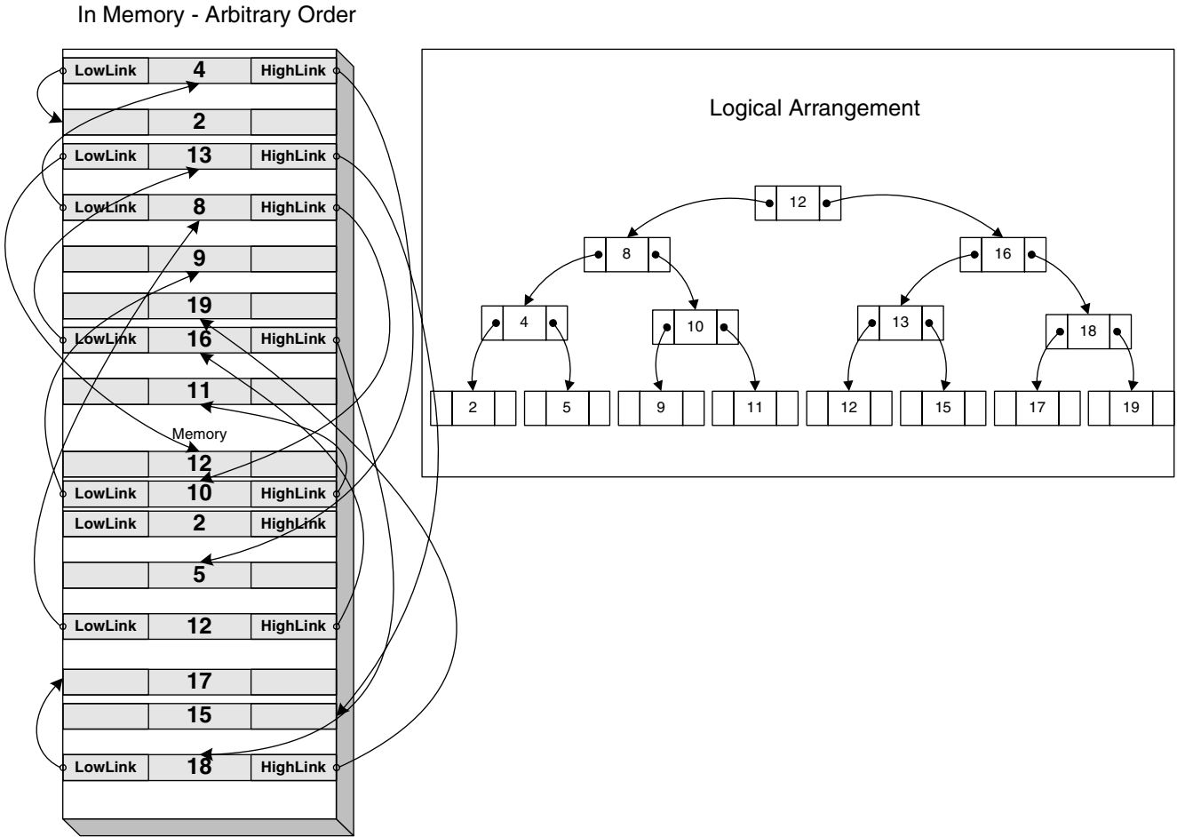
Figure C.4 Binary tree layout: in memory and logically.
