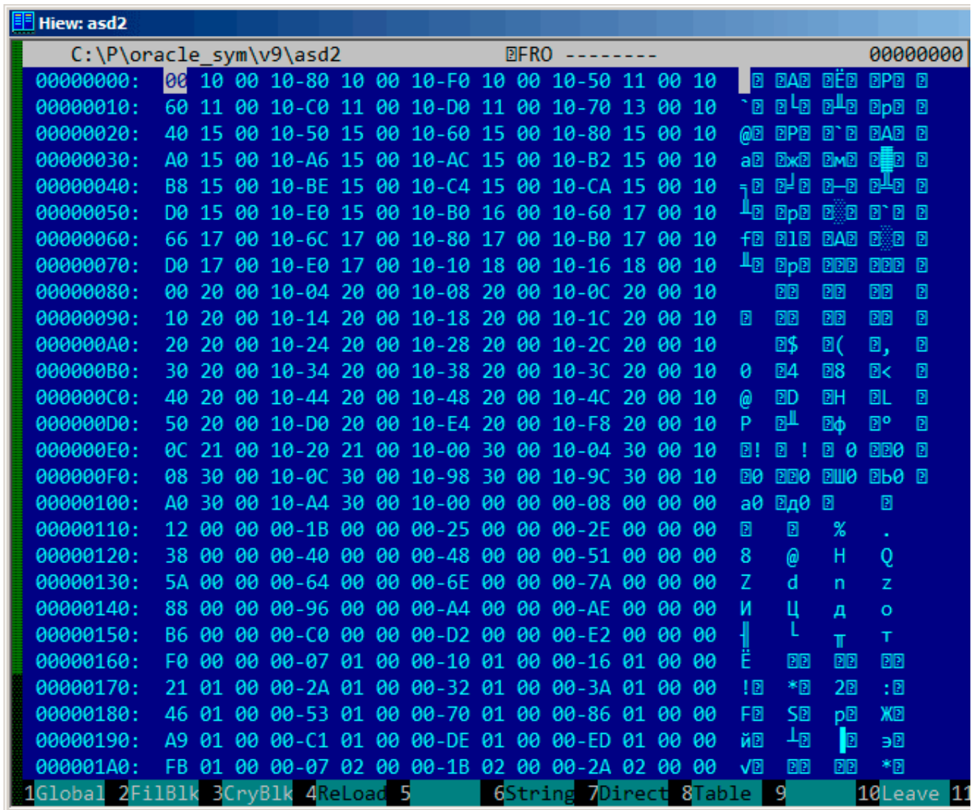
Figure 9.24: Binary block
