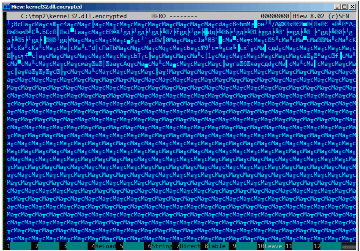
Figure 9.5: “Encrypted” file
