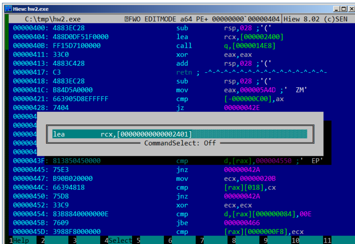
Figure 1.3: Hiew
