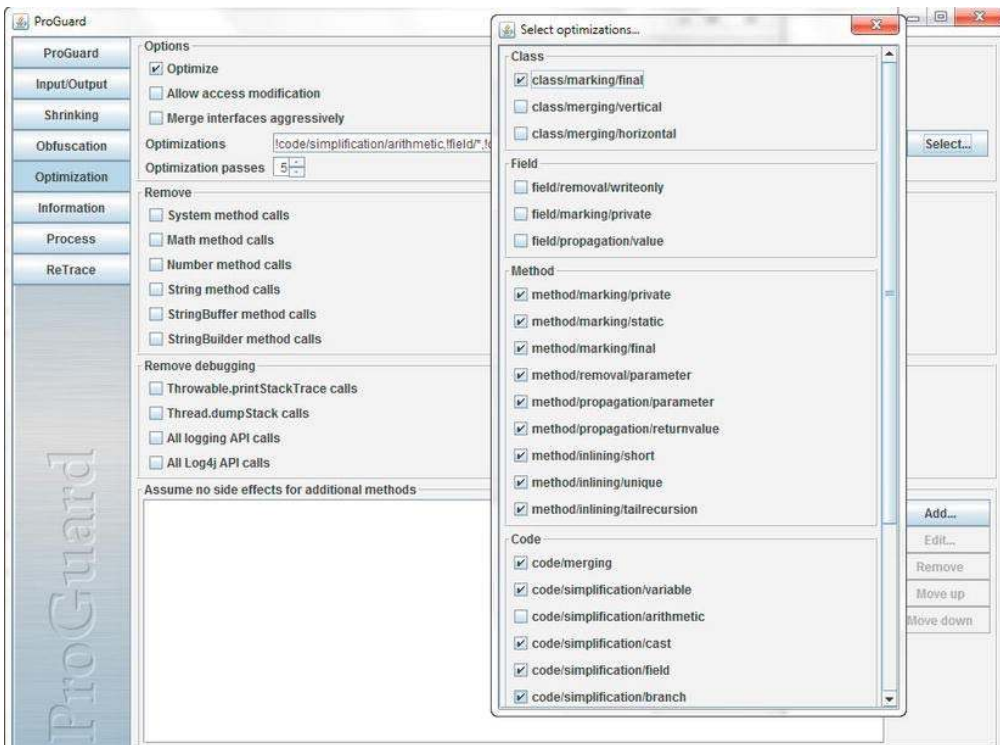
Figure 7-2. ProGuard GUI
