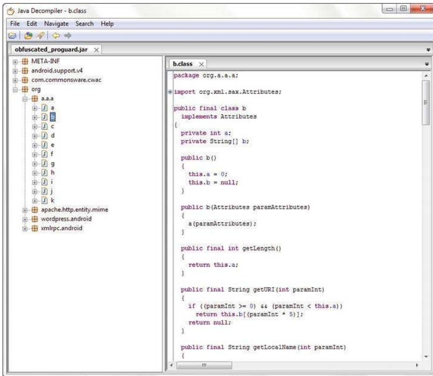
Figure 4-8. ProGuard-protected code
