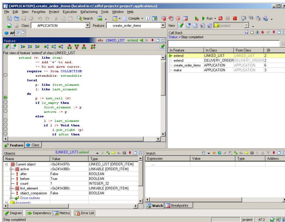
A debugger session with EiffelStudio
