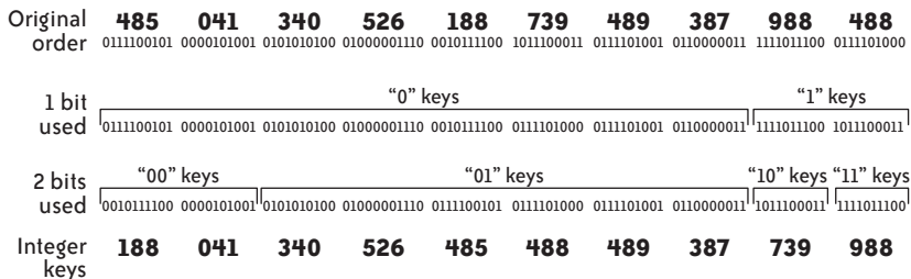
FIGURE 8-8. Radix exchange sort—two phases
