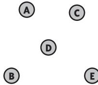
(b) Choose node A as root
