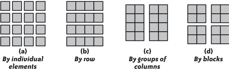
FIGURE 2-2. Array decomposition examples
