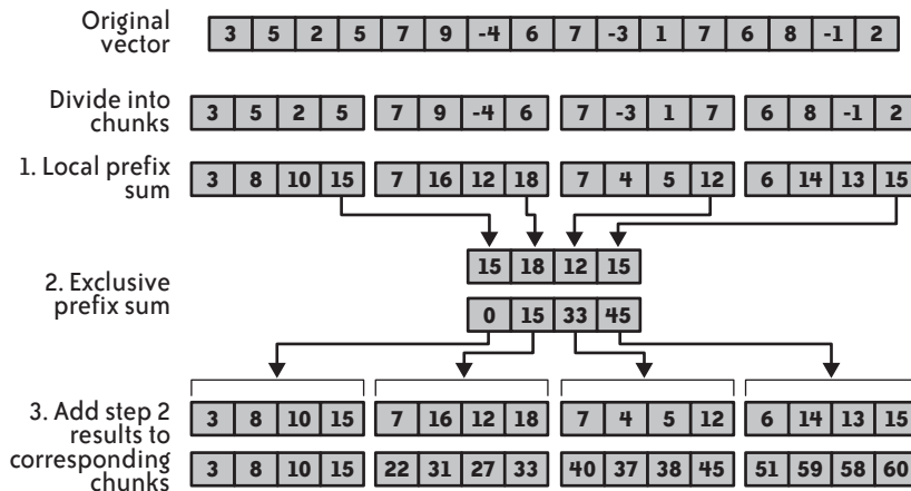
FIGURE 6-5. Prefix scan algorithm example
