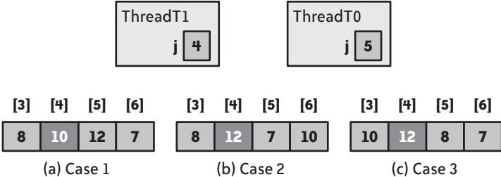
FIGURE 8-2. BubbleSort() interleaving cases
