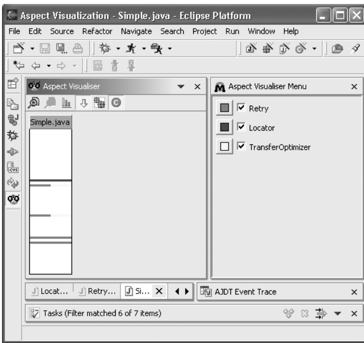
Figure 12-1. Three aspects for client/server communication
