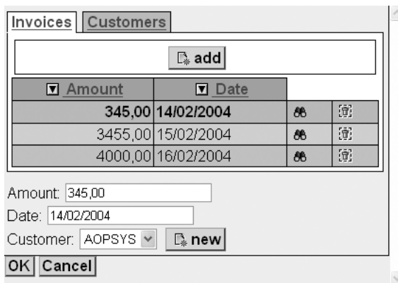
Figure 4-4. HTML/servlet version of the GUI aspect
