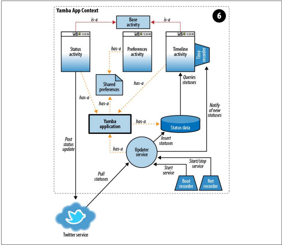
Figure 11-1. Yamba completion
