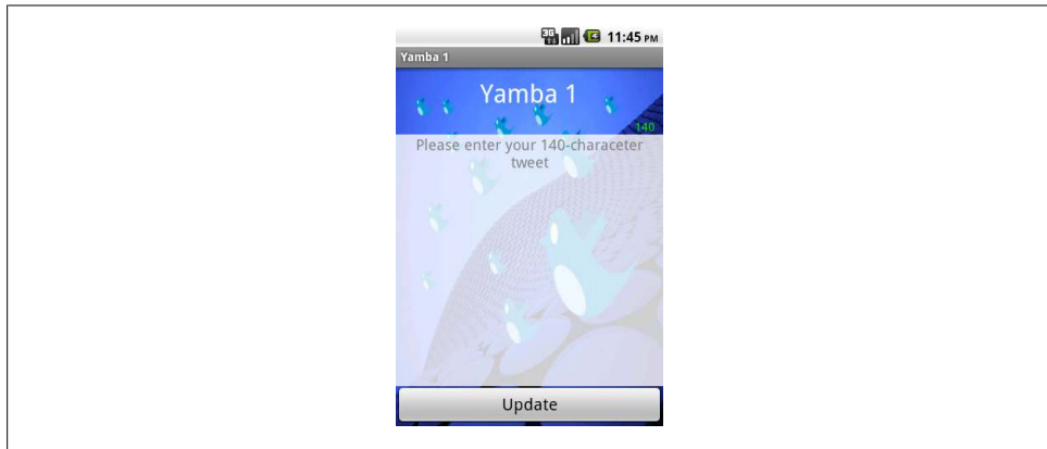
Figure 6-17. StatusActivity
