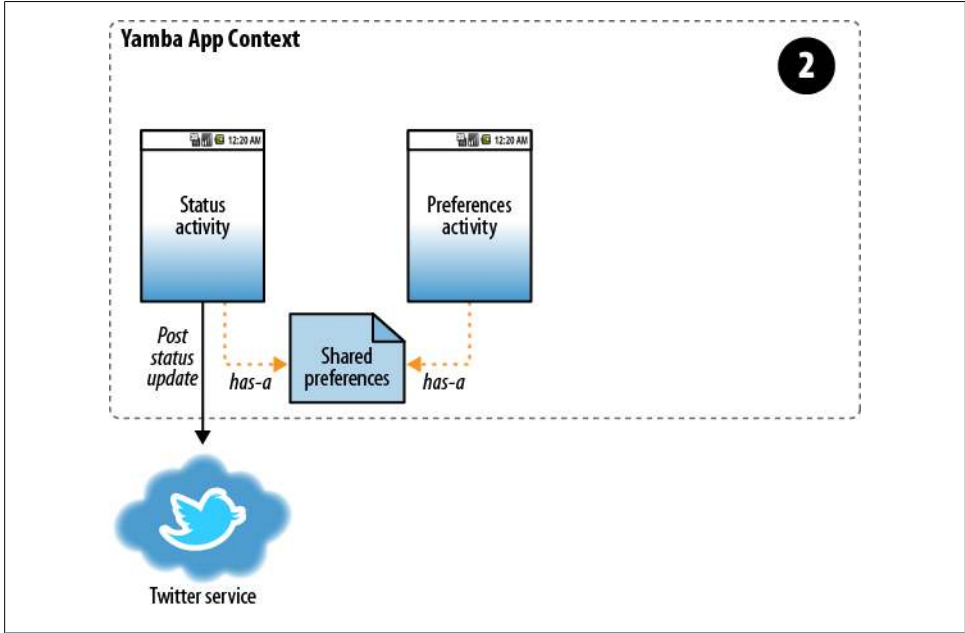
Figure 7-6. Yamba completion
