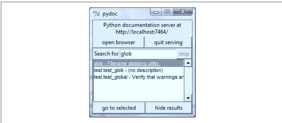
Figure 15-1. The Pydoc top-level search engine GUI: type the name of a module you want documentation for, press Enter, select the module, and then press “go to selected” (or omit the module name and press “open browser” to see all available modules).
