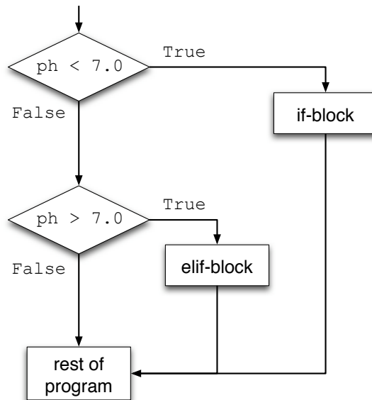
Figure 6.5: elif statement
