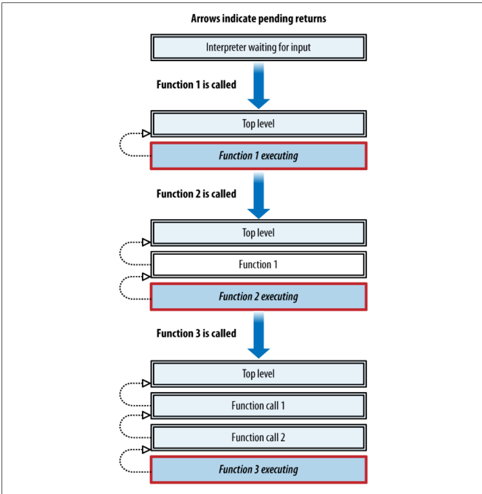
Figure 2-3. Function calls
