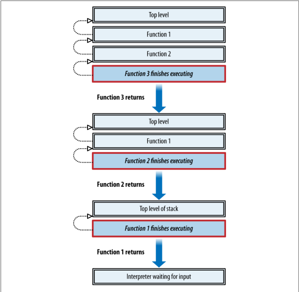
Figure 2-4. Function returns
