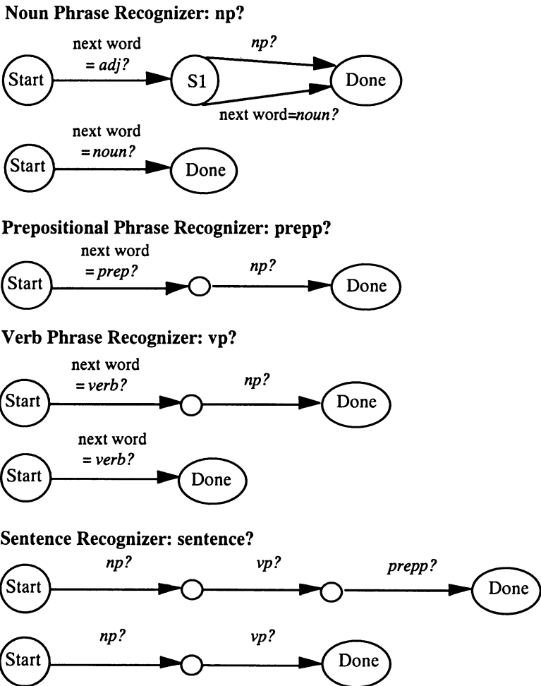
Figure 8.2. "Bubble diagram" for an Augmented Transition Network (ATN) parser
