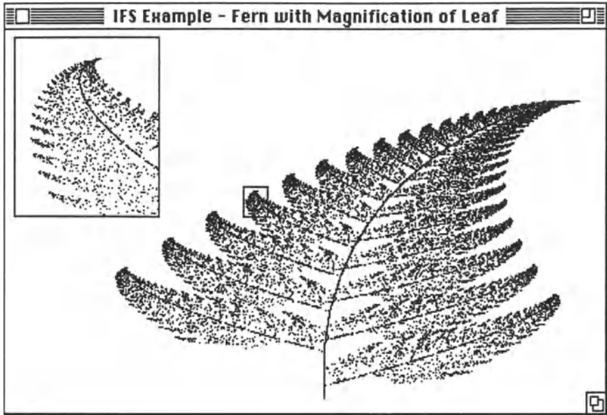
Figure 14.4. A Fern Produced by an IFS.
