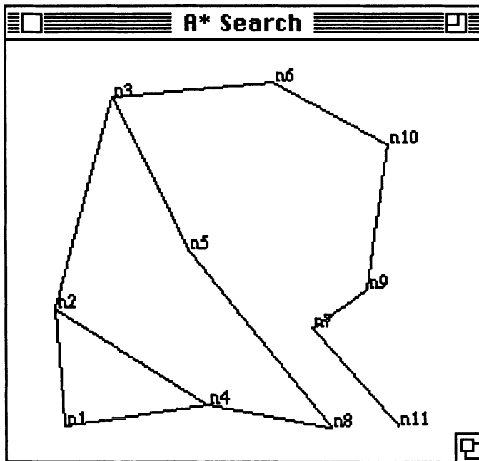
Figure 11.1. Sample Network with 11 Nodes and 12 Edges
