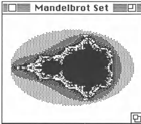
Figure 14.1. Low-resolution Mandelbrot Set Plot. This was produced by setting num-x-cells to 90 and num-y-cells .
