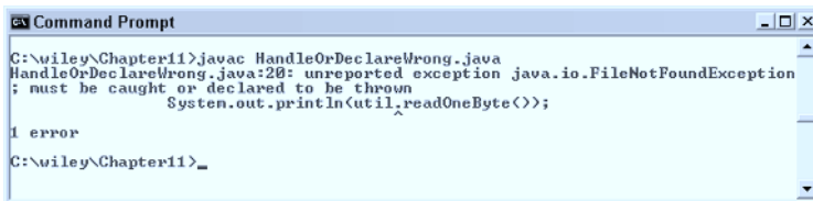
Figure 11.6 The compiler is enforcing the Handle or Declare Rule.
