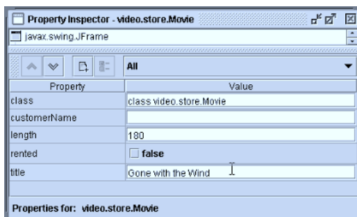
Figure 19.11 All the properties of the Movie bean.
