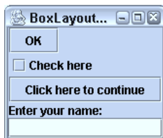
Figure 12.9 Output of the BoxLayoutDemo program.
