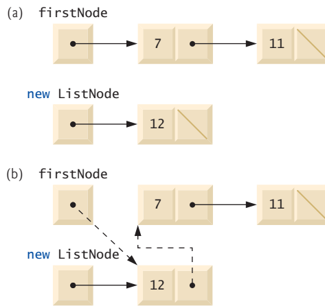
Fig. 22.6 | Graphical representation of operation insertAtFront .
