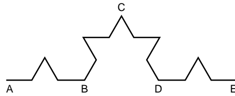
FIGURE 18.41 The Koch curve continued
