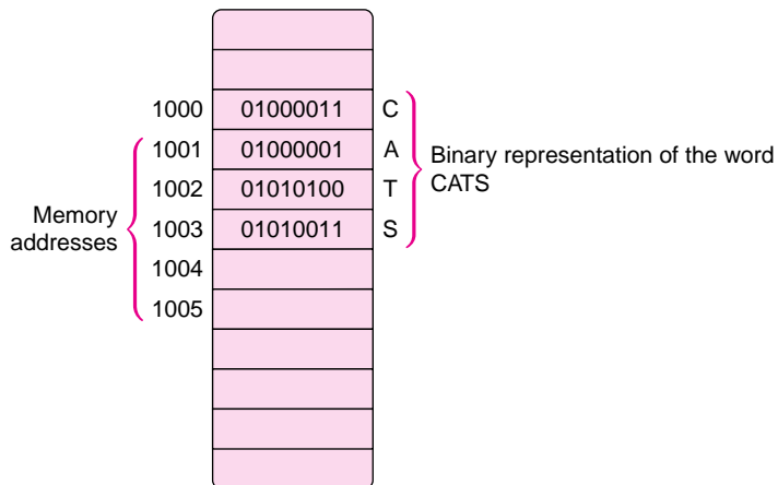
FIGURE 1.1 Primary memory
