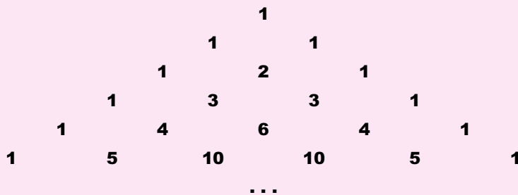
FIGURE 8.18 Pascal's triangle
