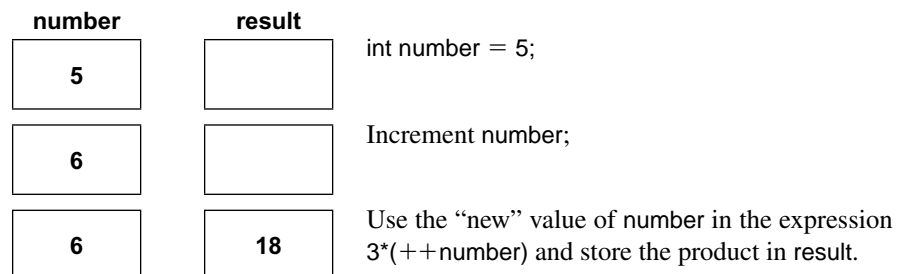
FIGURE 3.6 Prefix operator
