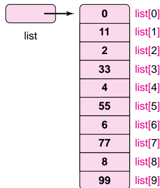
FIGURE 7.7 The array list holds 10 numbers
