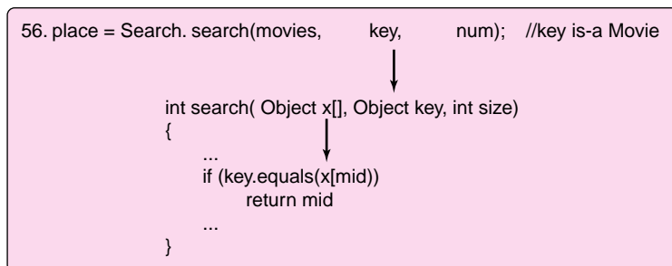
FIGURE 13.7 A call to search(...) and then to equals(...)
