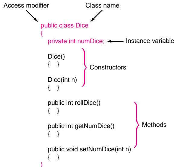
FIGURE 10.2 The Dice class
