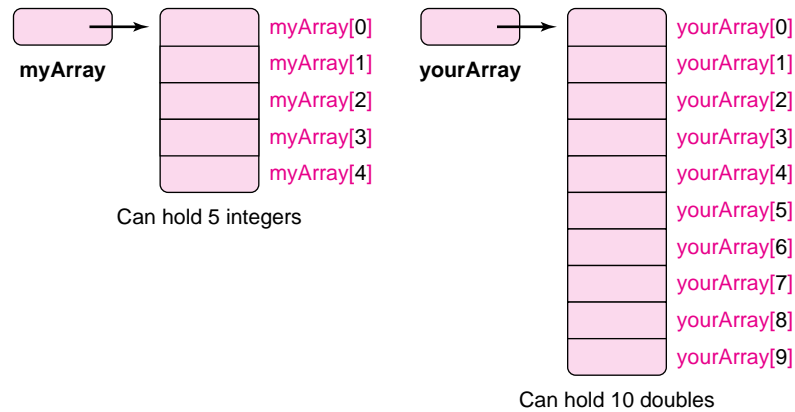
FIGURE 7.2 Two arrays myArray and yourArray
