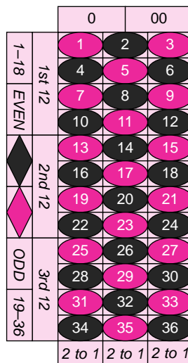
FIGURE 7.8 A roulette board has numbers 1 through 36 as well as 0 and 00
