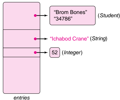
FIGURE 16.2 An ArrayList can refer to objects of different classes
