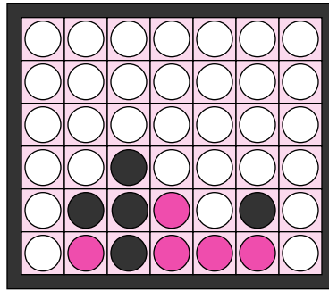
FIGURE 7.44 Connect Four
