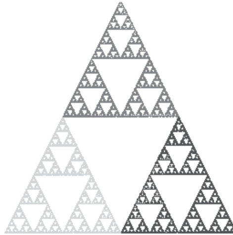
FIGURE 18.27 Sierpinski's Triangle
