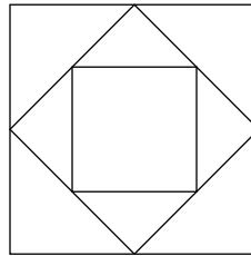
FIGURE 18.38 A square inside a square inside a square
