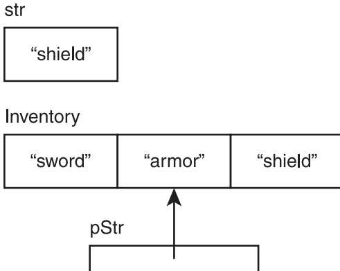
Figure 7.6 str is a new string object, totally independent from inventory .
