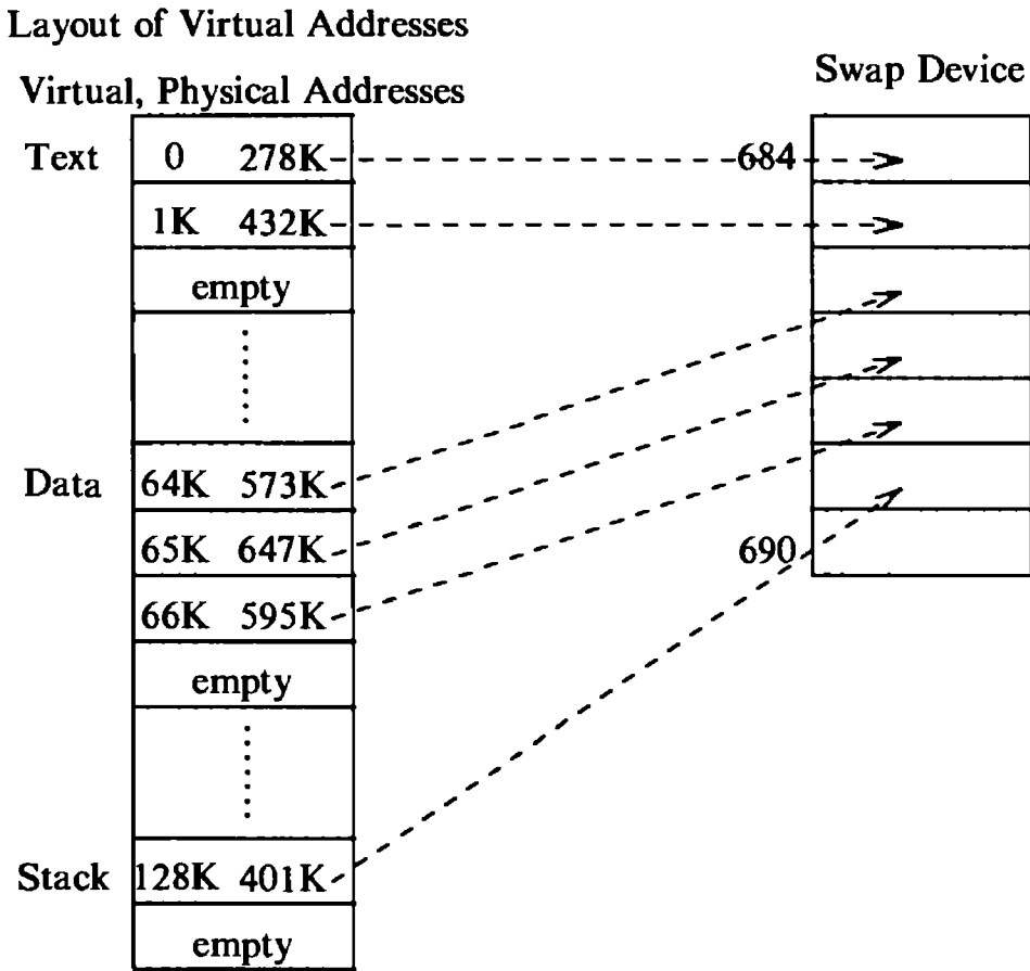
Figure 9.6. Mapping Process Space onto the Swap Device
