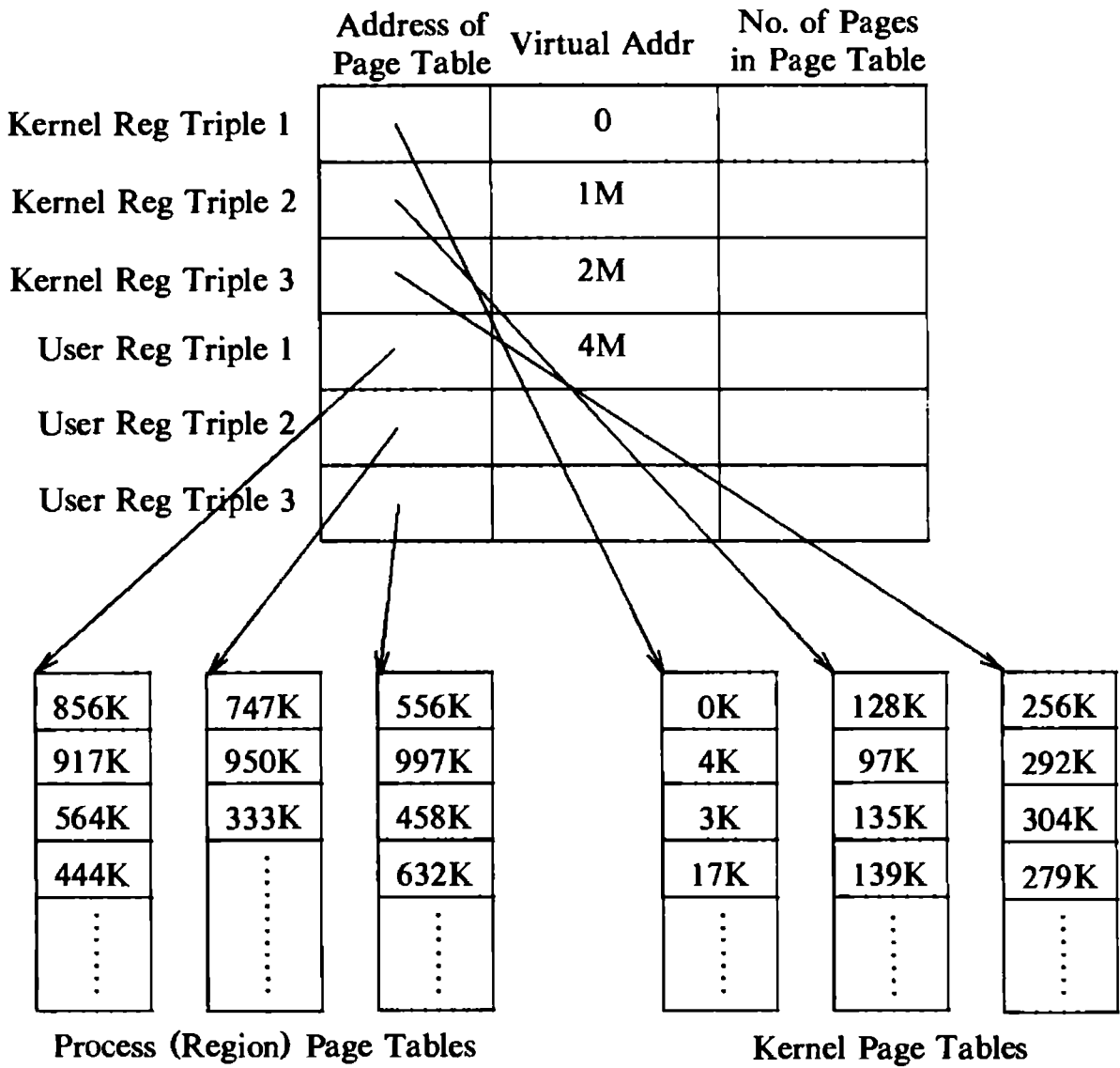
Figure 6.6. Changing Mode from User to Kernel
