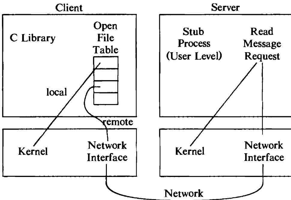
Figure 13.9. Formulation of File Service Requests
