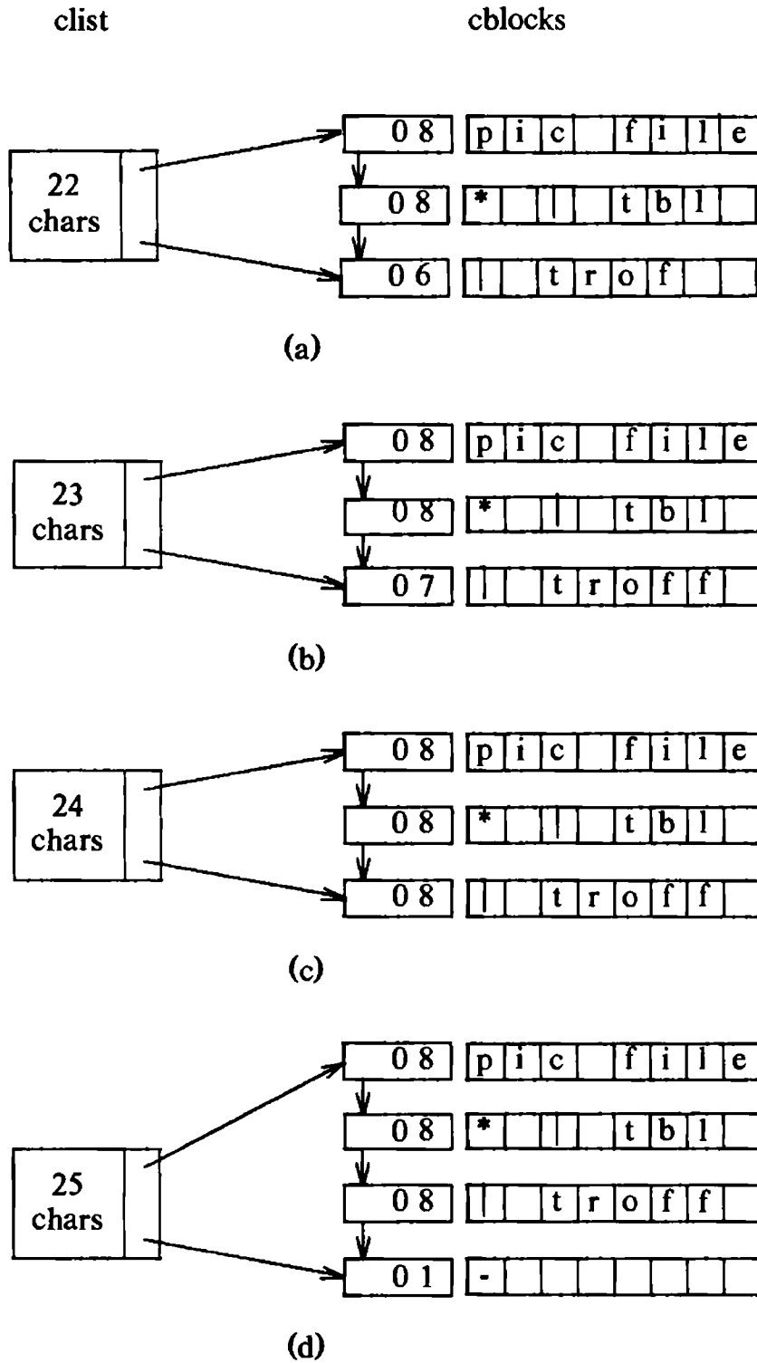
Figure 10.12. Placing a Character on a Clist
