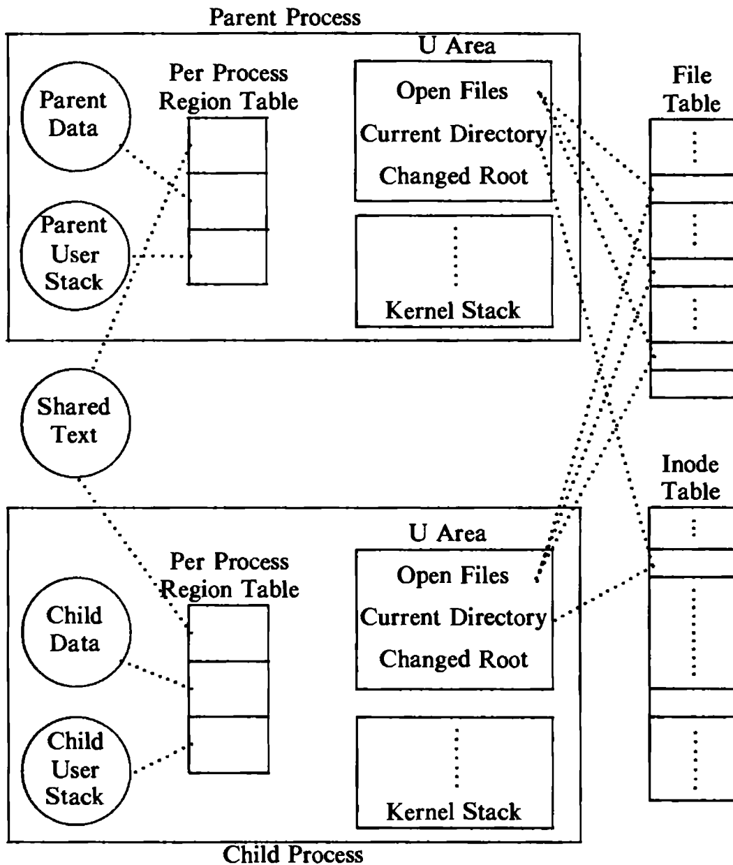
Figure 7.3. Fork Creating a New Process Context
