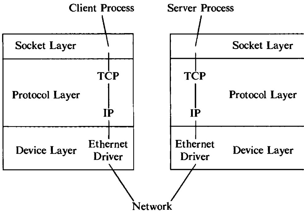
Figure 11.18. Sockets Model
