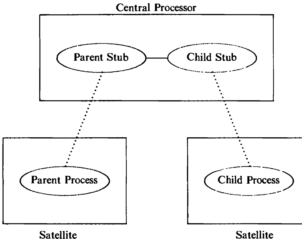
Figure 13.6. Fork on a Satellite Processor
