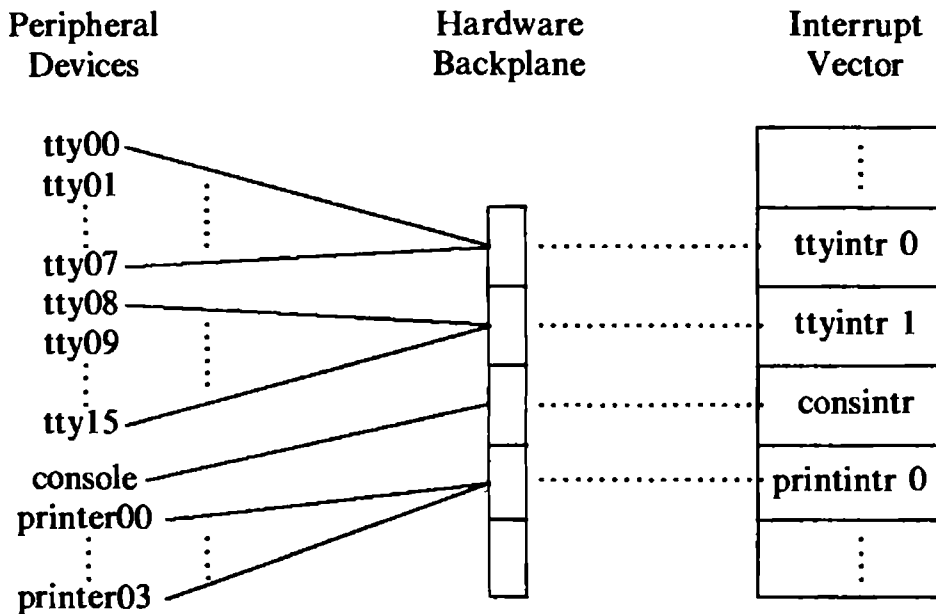
Figure 10.6. Device Interrupts
