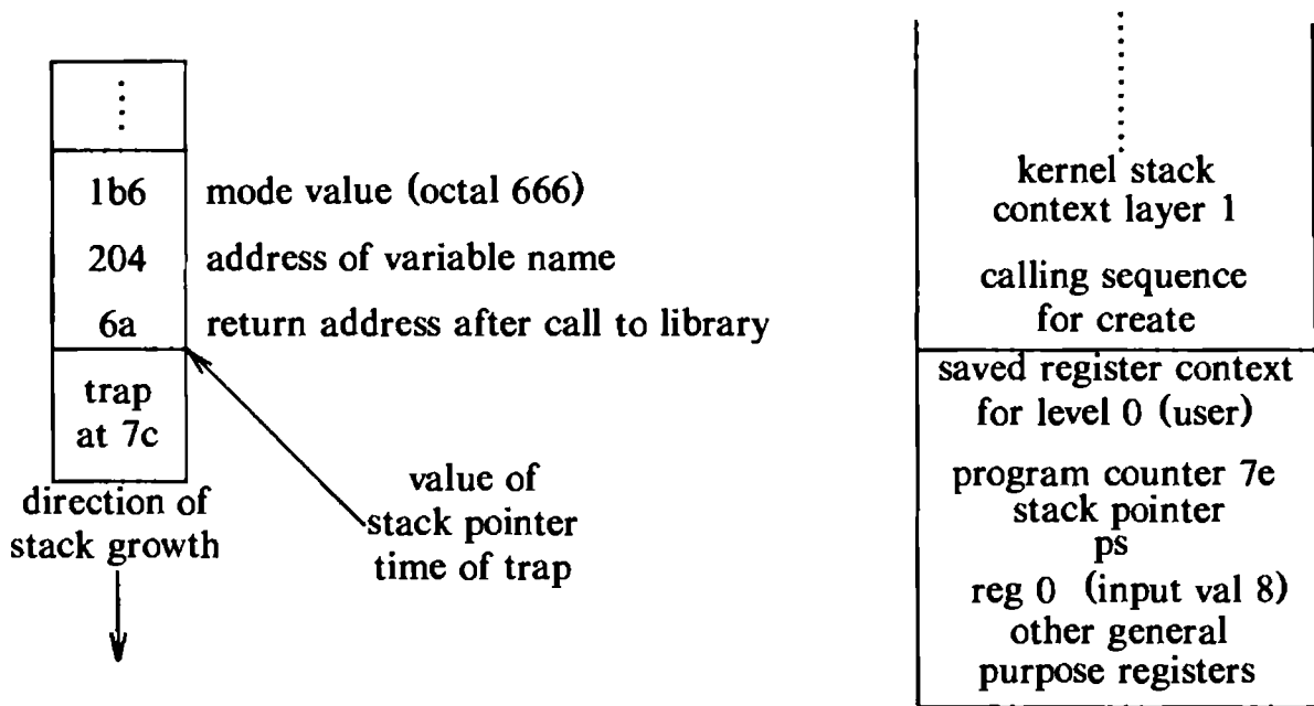
Figure 6.14. Stack Configuration for Creat System Call
