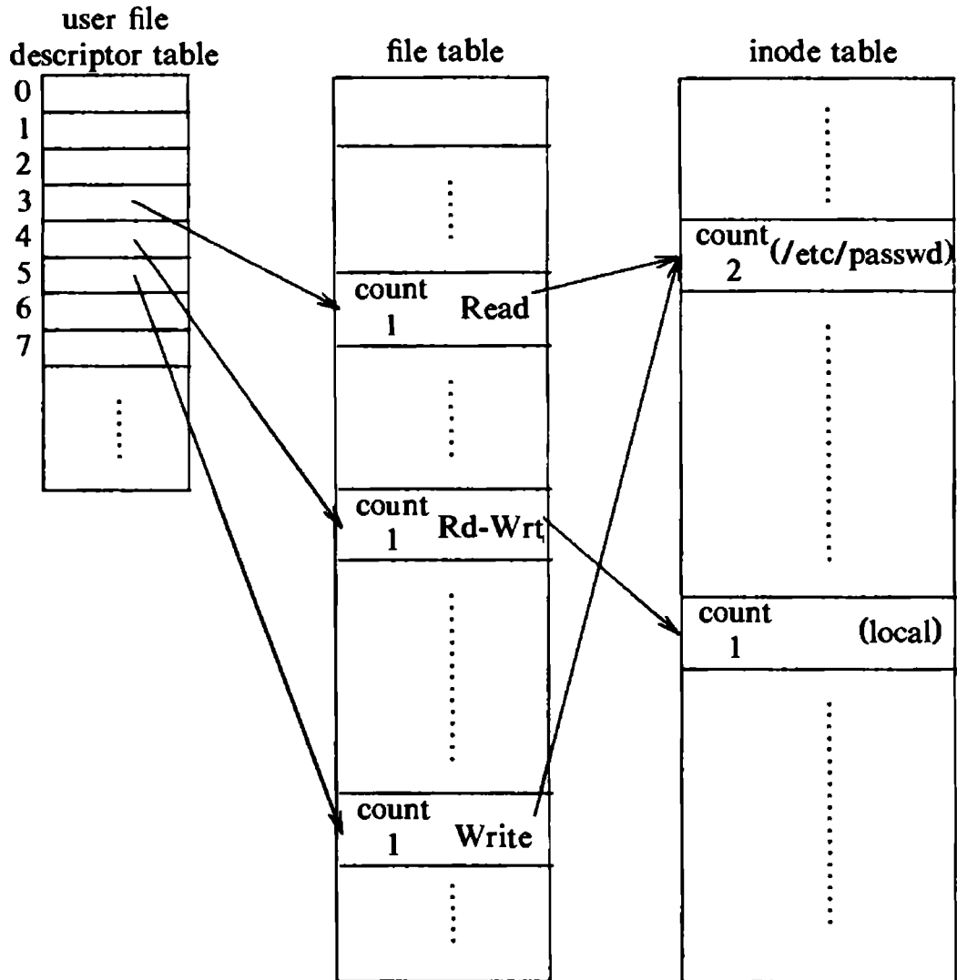
Figure 5.3. Data Structures after Open
