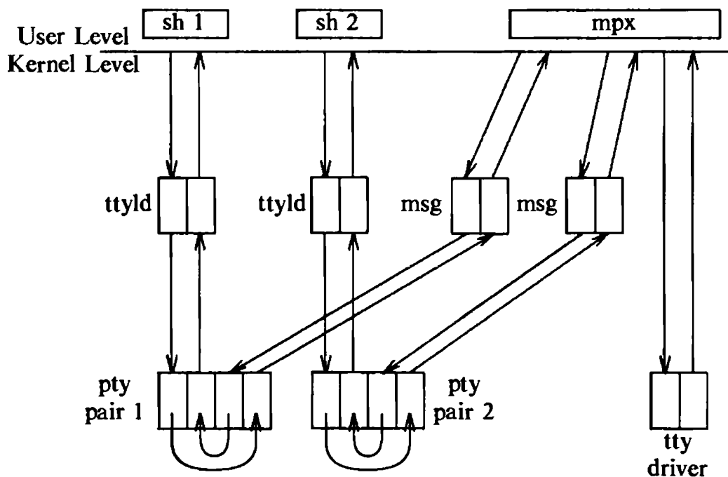
Figure 10.23. Windowing Virtual Terminals on a Physical Terminal
