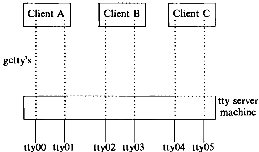
Figure 13.13. A Terminal Server Configuration
