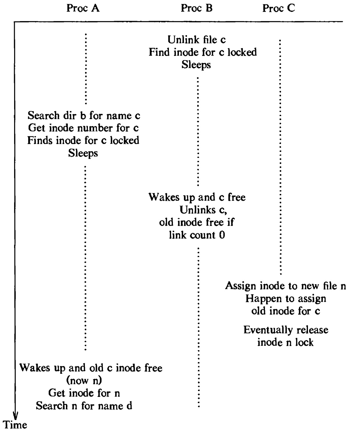
Figure 5.32. Unlink Race Condition
