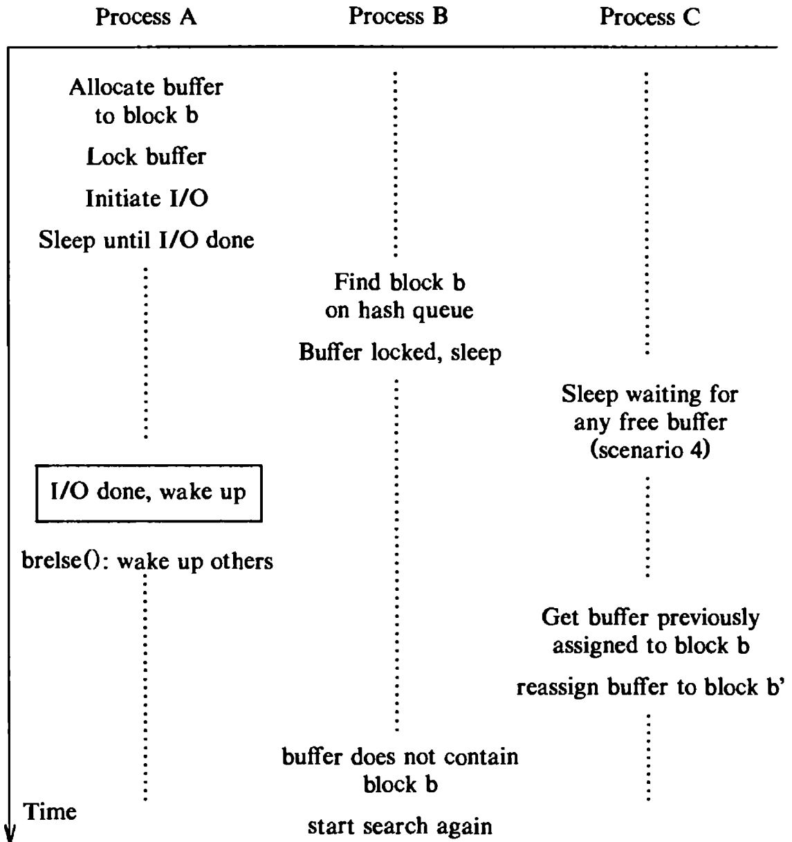
Figure 3.12. Race for a Locked Buffer
