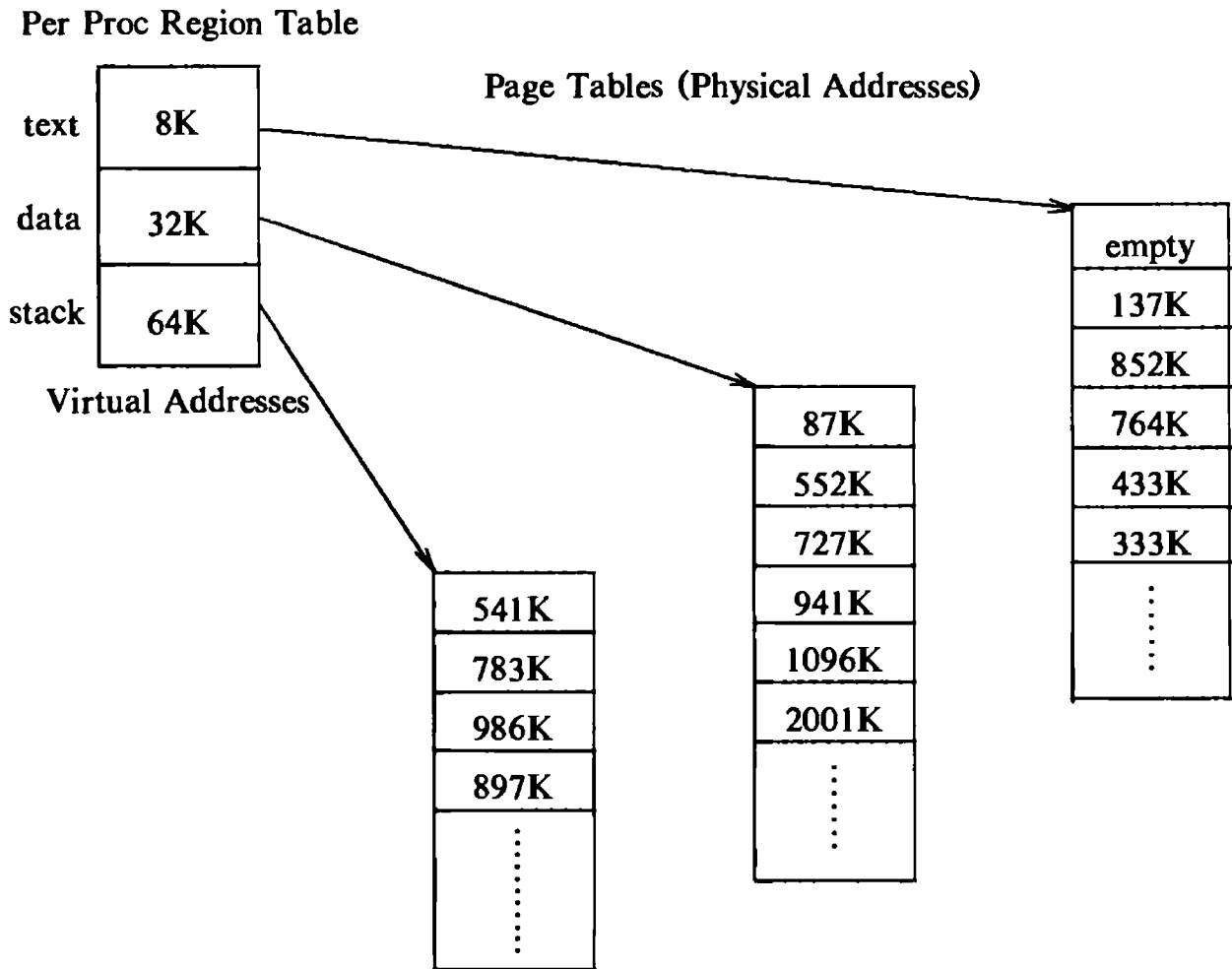
Figure 6.5. Mapping Virtual Addresses to Physical Addresses
