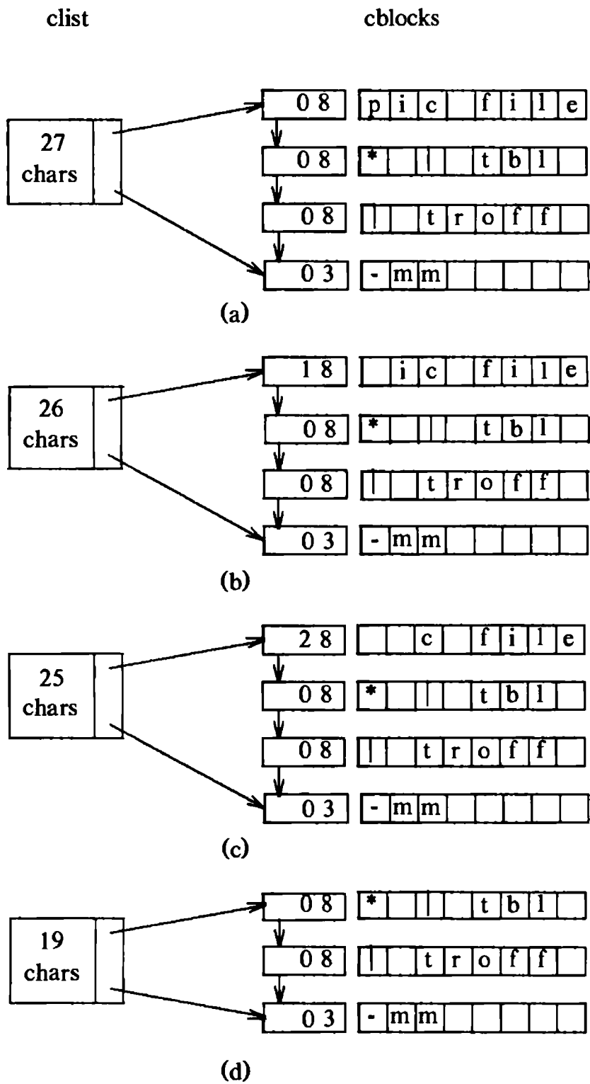
Figure 10.11. Removing Characters from a Clist
