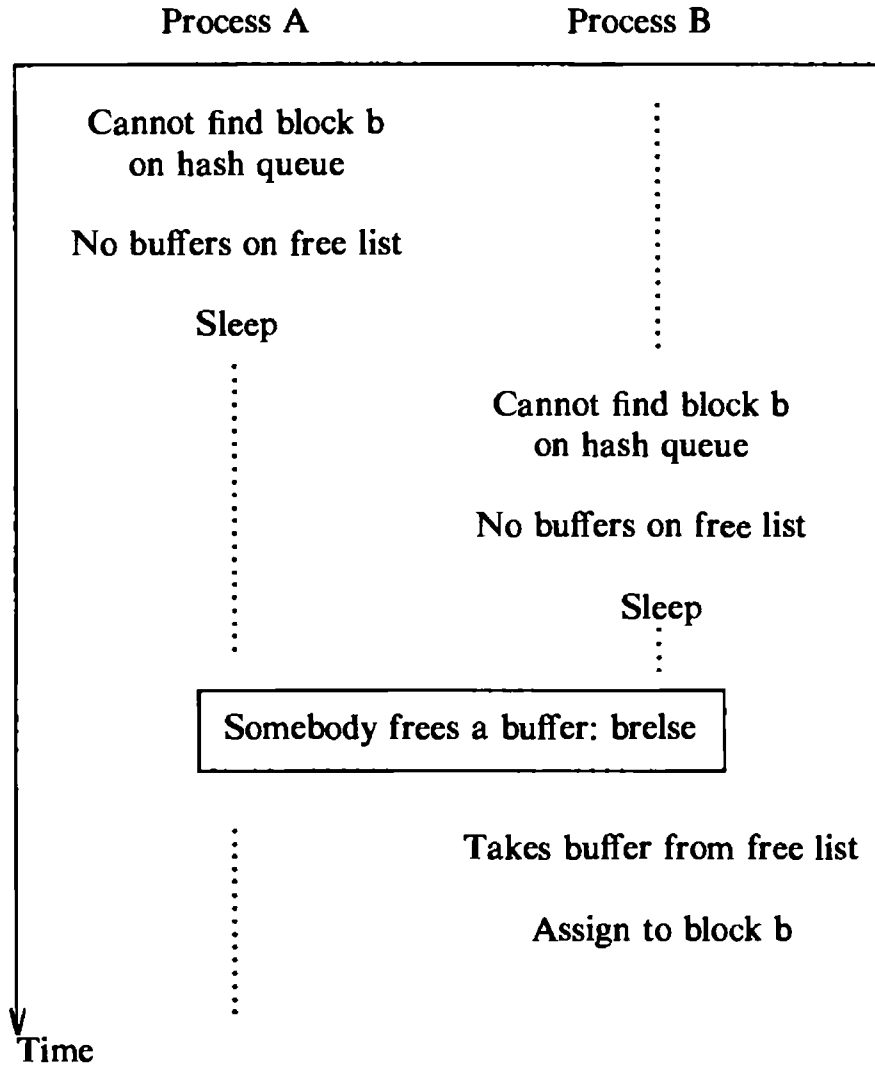
Figure 3.10. Race for Free Buffer
