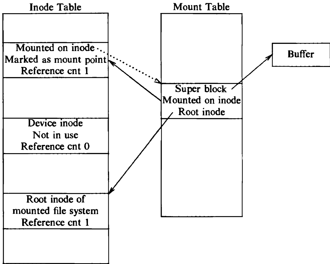
Figure 5.24. Data Structures after Mount
