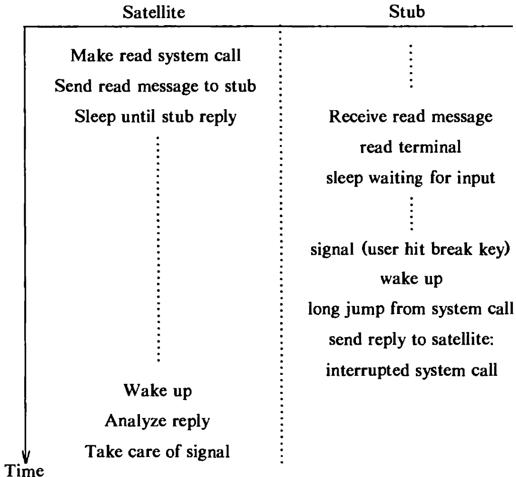
Figure 13.8. Interrupt in Middle of a System Call
