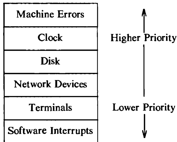
Figure 1.6. Typical Interrupt Levels
