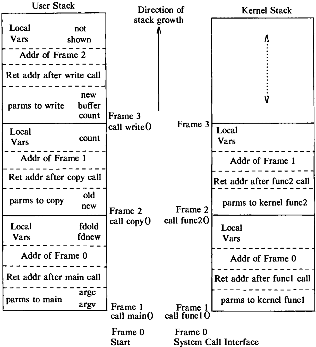
Figure 2.4. User and Kernel Stack for Copy Program
