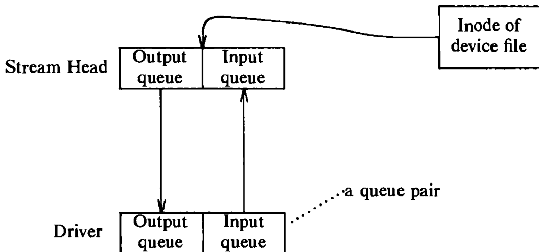
Figure 10.20. A Stream after Open
