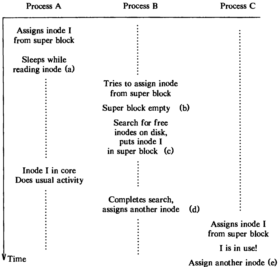
Figure 4.16. Race Condition in Assigning Inodes
