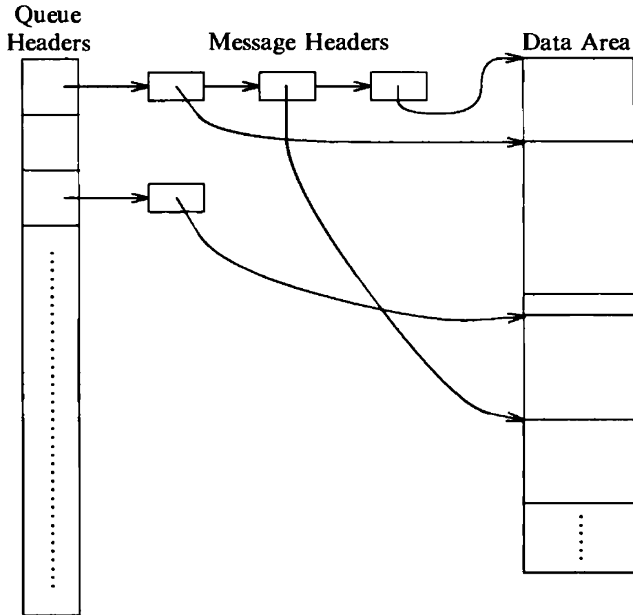
Figure 11.5. Data Structures for Messages
