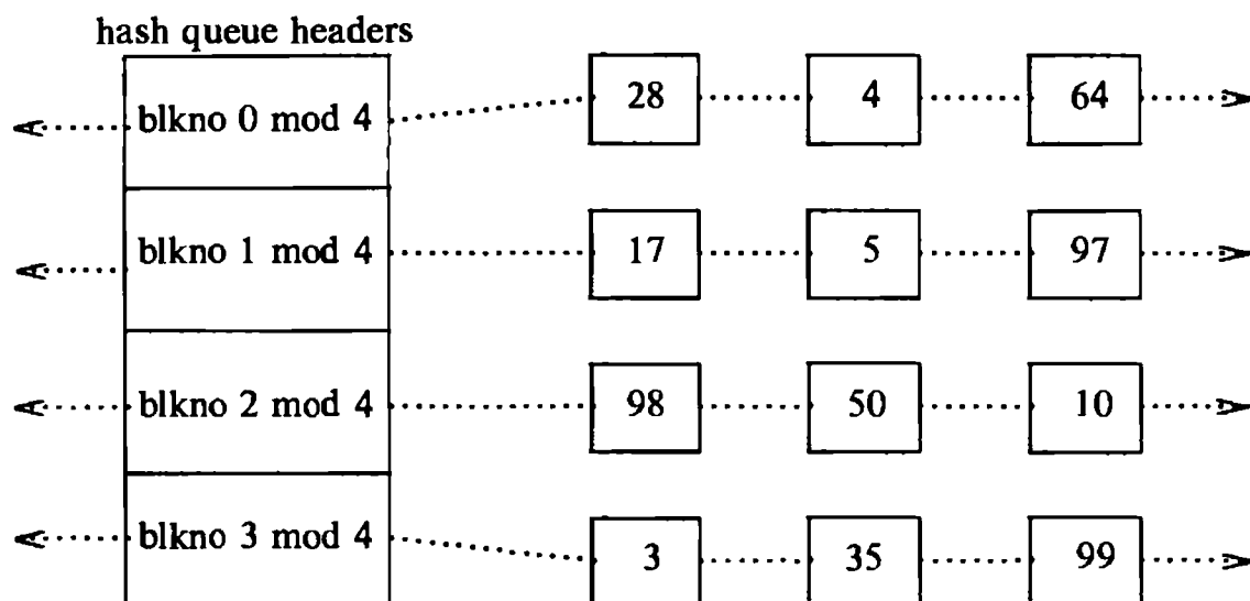
Figure 3.3. Buffers on the Hash Queues
