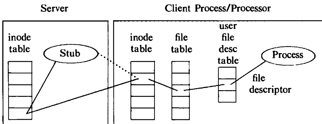
Figure 13.11. Opening a Remote File
