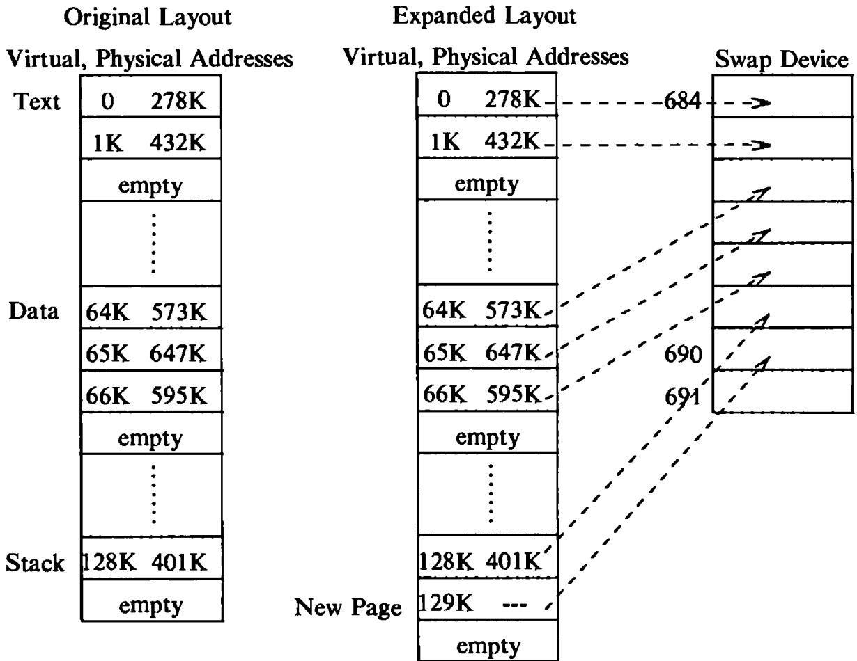
Figure 9.8. Adjusting Memory Map for Expansion Swap
