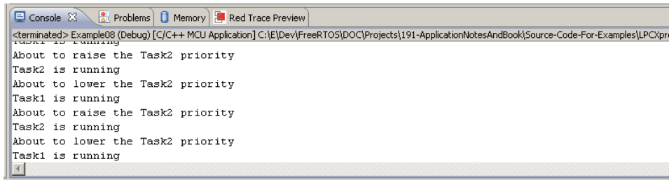
Figure 15. The output produced when Example 8 is executed
