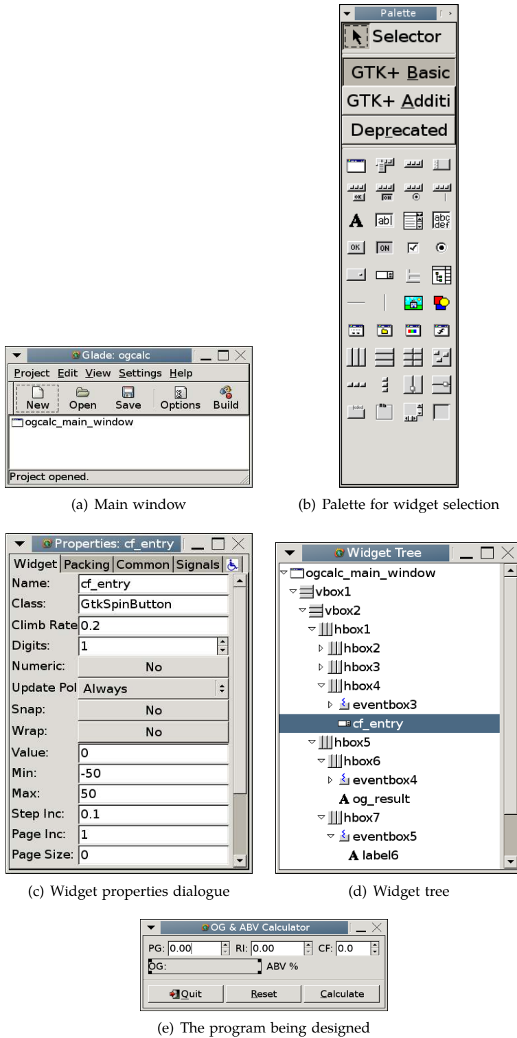
Figure 8: The Glade user interface designer.
