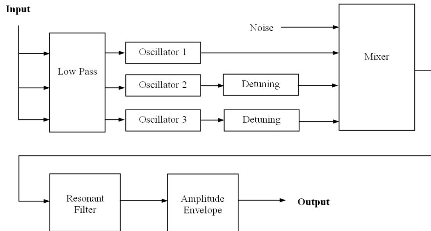
Figure 21: System diagram for Minimooq emulator.
