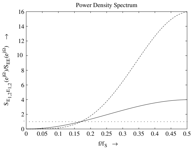
Figure 2.29 Spectrum shaping ( S_{EE}(e^{j\Omega}) \cdots, S_{E_1E_1}(e^{j\Omega}) —, S_{E_2E_2}(e^{j\Omega}) - - -).
