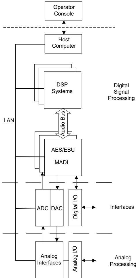
Figure 4.24 Audio system.
