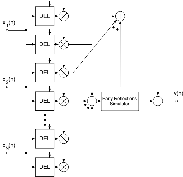
Figure 6.10 Multichannel application.
