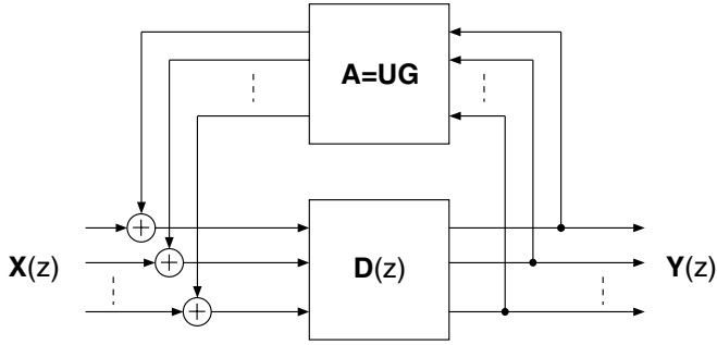
Figure 6.25 Feedback system.
