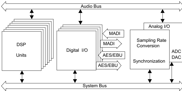
Figure 4.26 Subsystem.
