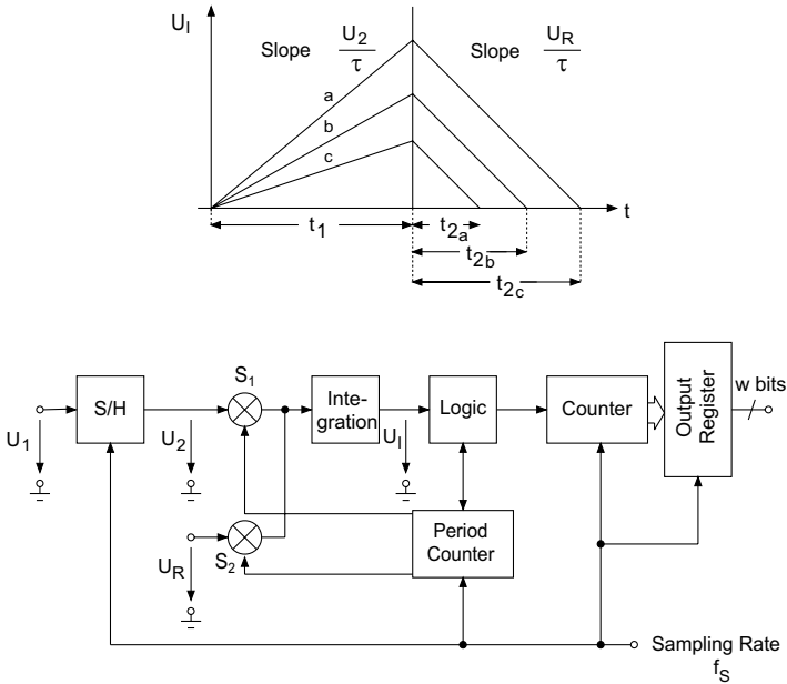
Figure 3.36 Dual-slope AD converter.
