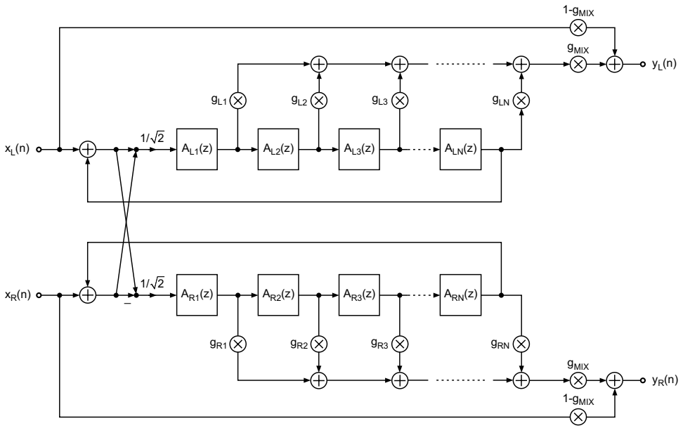
Figure 6.31 Stereo room simulator with absorbent all-pass systems [Dah00].
