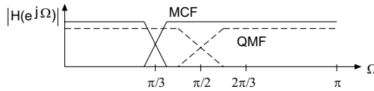
Figure 5.63 Two-band decomposition.
