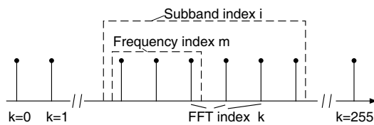
Figure 9.18 Nomenclature of frequency indices.
