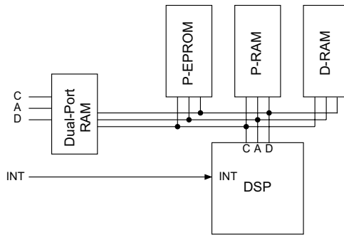
Figure 4.15 Control over a dual-port RAM and interrupt.
