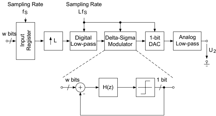
Figure 3.49 Delta-sigma DA converter.
