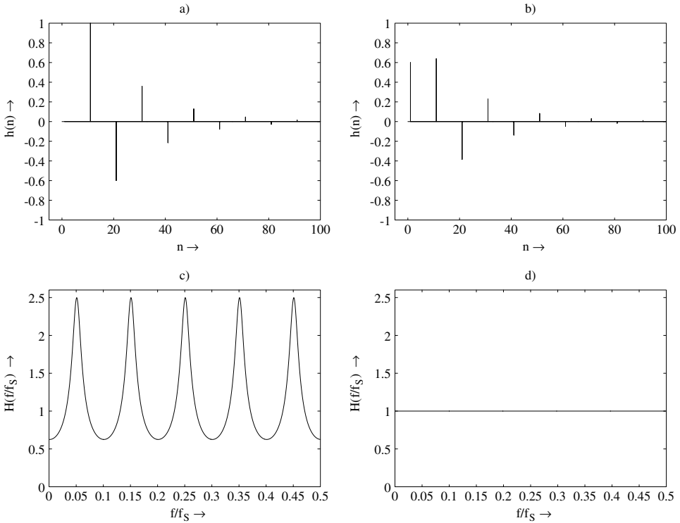
Figure 6.15 (a) Impulse response of a comb filter ( M = 10 , g = -0.6 ). (b) Impulse response of an all-pass filter ( M = 10 , g = -0.6 ). (c) Frequency response of a comb filter. (d) Frequency response of an all-pass filter.
