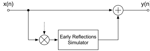
Figure 6.5 Simulation of early reflections.
