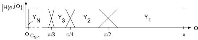
Figure 5.62 Octave-frequency bands.
