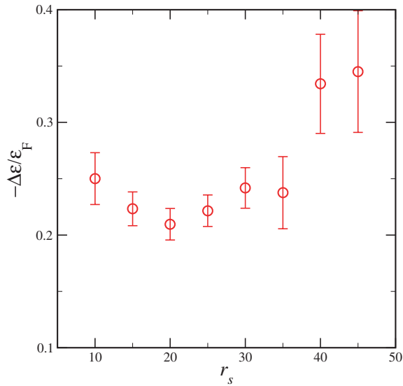
Fig. 10.3 The energy difference per particle \Delta\epsilon between the resonating-pair liquid and Fermi liquid measured in terms of the Fermi energy ( \epsilon_F = k_F^2/2 ) of the noninteracting system. The total number of particles used in all the simulations here is N = 58 . The largest difference obtained in the region shown for a spin-polarized liquid or Wigner crystal is on the order of, or smaller than, 0.1, not enough to make one of them a preferable state in the region shown.
