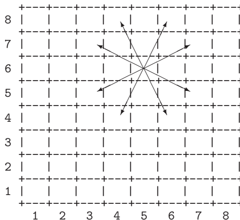
Figure 3.15: The Knight Moves One Step
