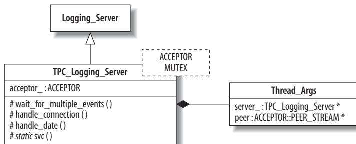
FIGURE 26-11. Thread-per-connection server interface
