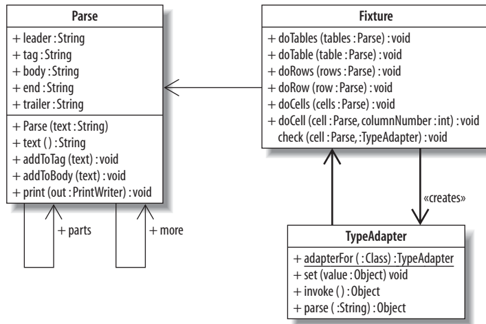
FIGURE 6-3. Relations among FIT classes
