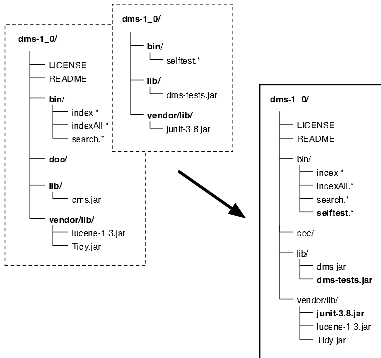
Figure 5.2: Adding Tests to a Standard Distribution
