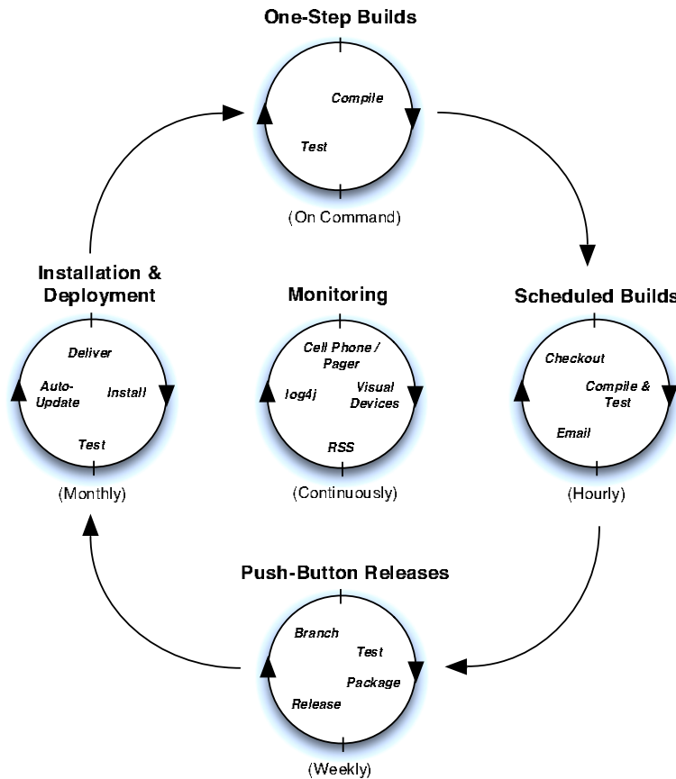
Figure 1.2: Automation Road Map
