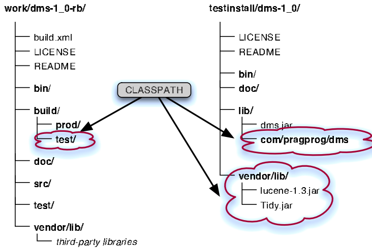
Figure 4.6: Testing the Release
