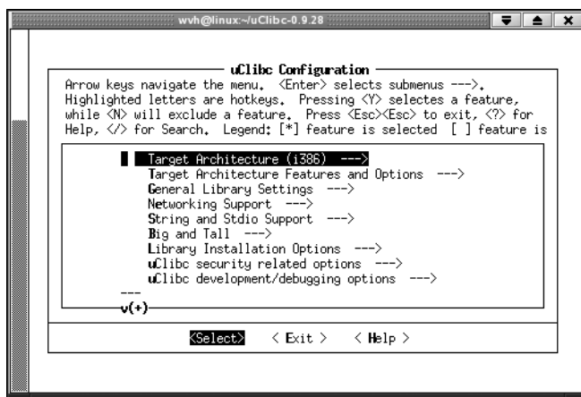
Figure 13-1. The main screen when configuring uClibc
