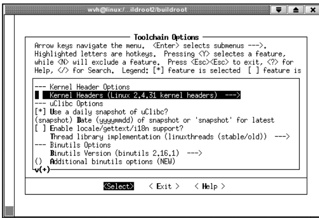
Figure 14-6. Setting general toolchain options
