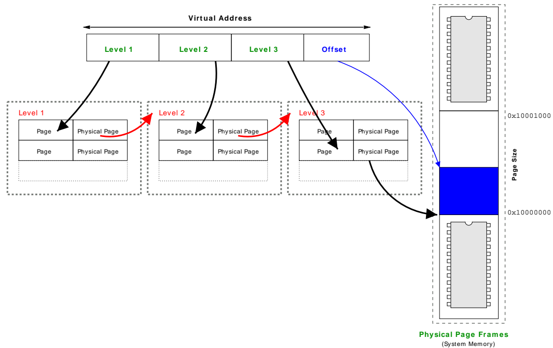
Figure 6.6. Linux Three Level Page Table
