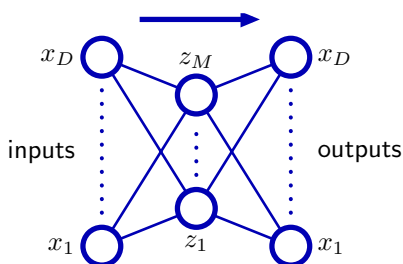
Figure 12.18 An autoassociative multilayer perceptron having two layers of weights. Such a network is trained to map input vectors onto themselves by minimization of a sum-of-squares error. Even with nonlinear units in the hidden layer, such a network is equivalent to linear principal component analysis. Links representing bias parameters have been omitted for clarity.
