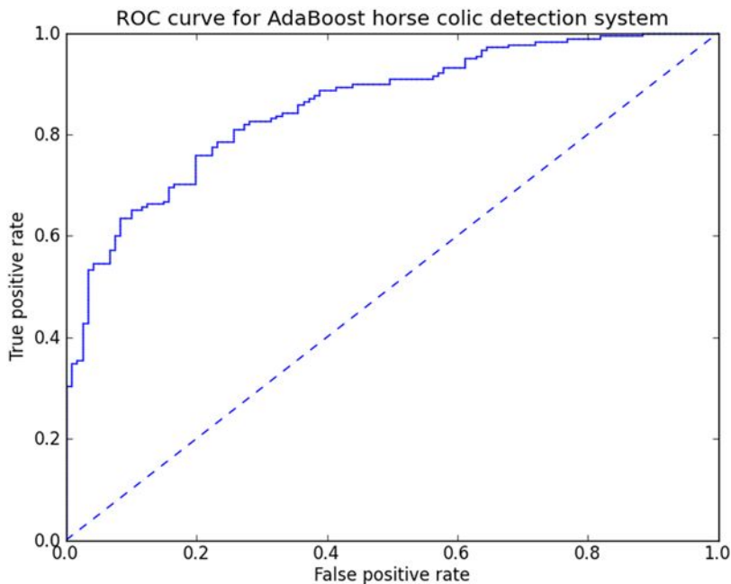
Figure 7.3 ROC for AdaBoost horse colic detection system using 10 decision stumps
