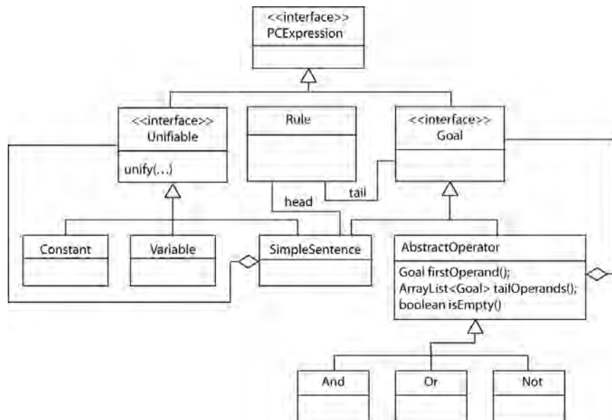
Figure 24.7. A Horn clause Rule representation as an instance of PCExpression.
