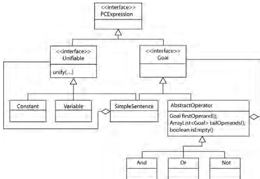
Figure 24.6. Classes and interfaces for a logic-based inference system.
