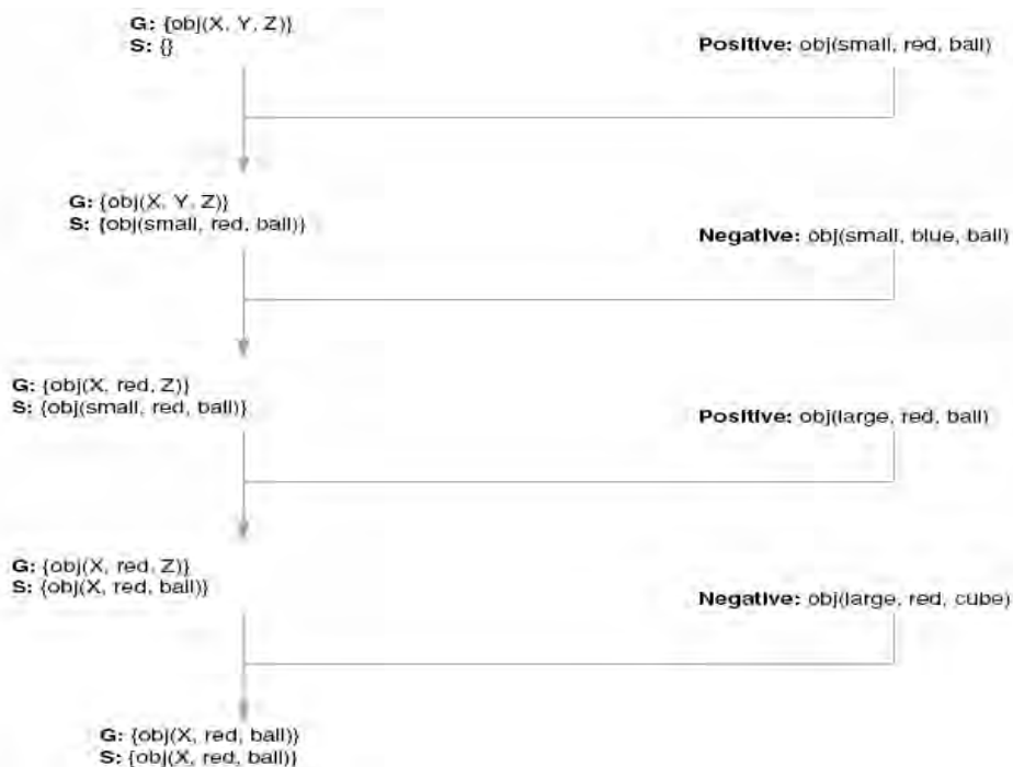
Figure 7.4. The candidate elimination algorithm learning the concept “red ball.”
