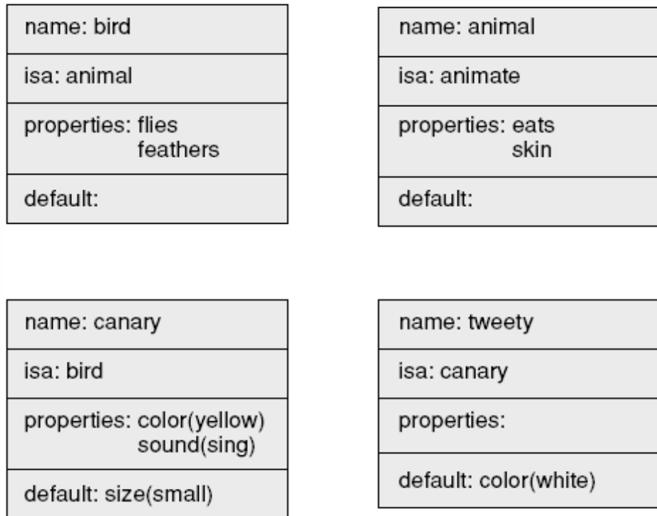
Figure 2.2 A frame system reflecting the Prolog code in the text.
