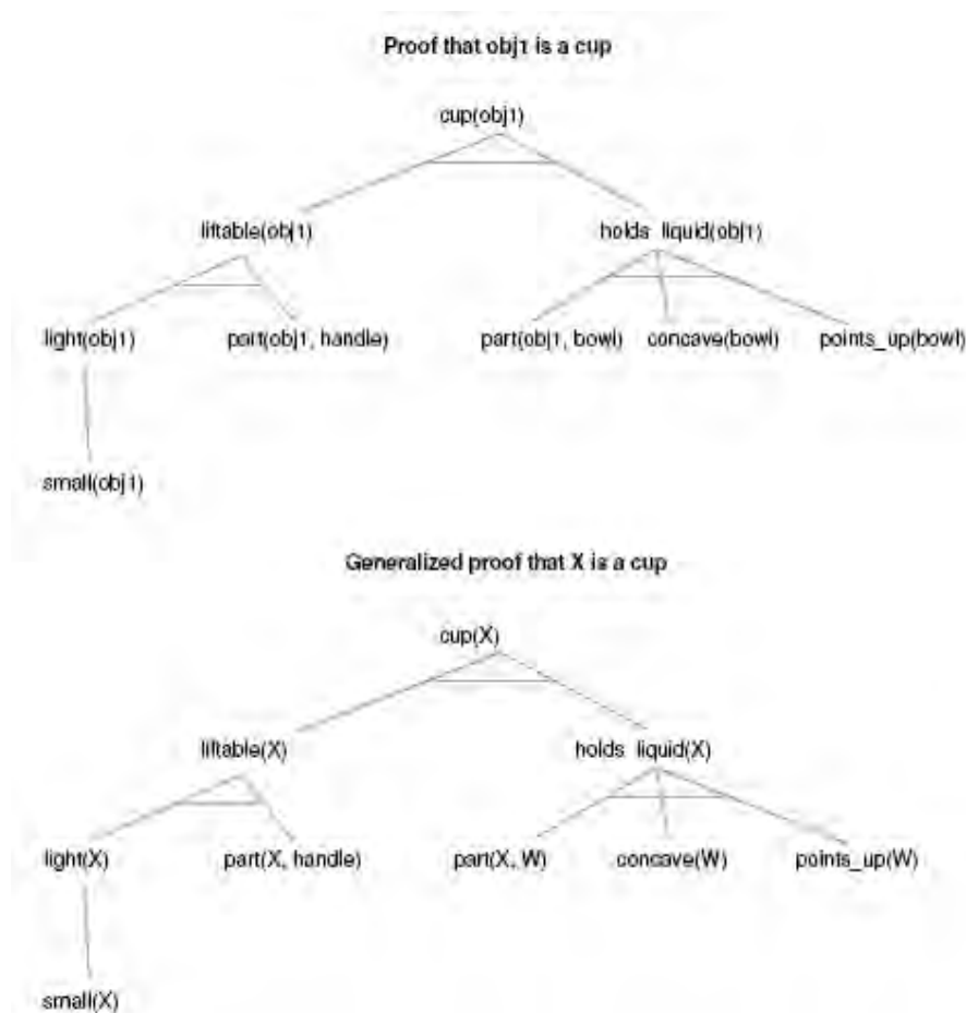
Figure 7.5. A specific (top) and generalized (bottom) proof that an object, X, is a cup.
