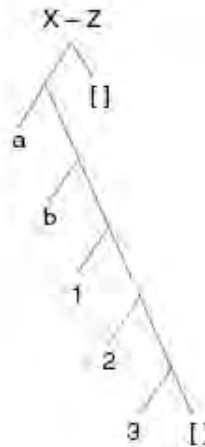
Figure 5.1 Tree diagrams: list concatenation using difference lists.
