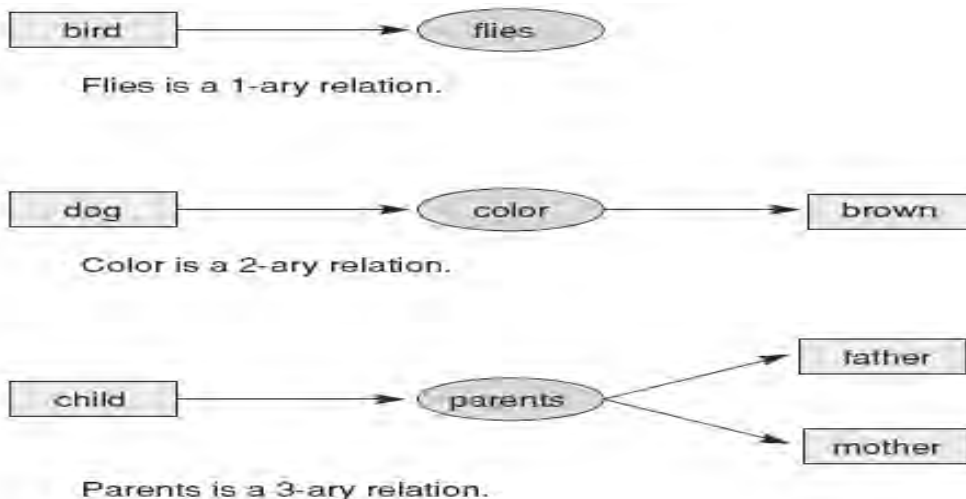
Figure 8.1. Conceptual graph relations with different arities.
