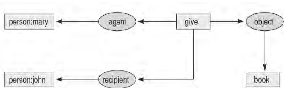
Figure 8.2. Conceptual graph of “Mary gave John the book.”
