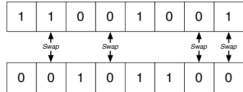
Figure 11 Uniform Crossover.
