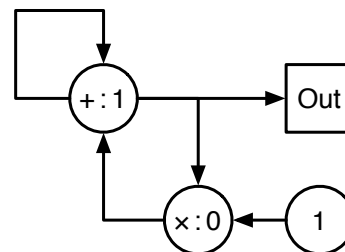
Figure 17 Neural Programming encoding of the Fibonacci Sequence (1, 1, 2, 3, 5, 8, 13, 21, 34, 55, 89, 144, 233, 377, 610, 987, etc.). See if you can work it out. The node "1" always emits a 1. The node "+ : 1" emits a 1 on the first timestep, then later emits the sum of its inputs. The node "x : 0" emits a 0 on the first timestep, then later emits the product of its inputs. The sequence is read at the node "Out".
