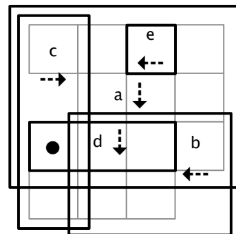
Figure 66 A sparse version of the optimal policy for the cockroach robot world, with five rules ( a..e ). Compare to Figure 63. The state marked \bullet is covered by three different rules ( a, c , and d ), with d being the most specific.
