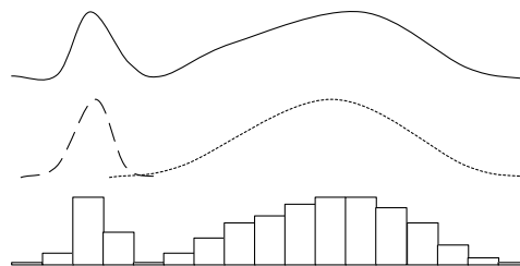
Figure 61 Gaussian and histogram representations of a 1-dimensional marginal distribution.
