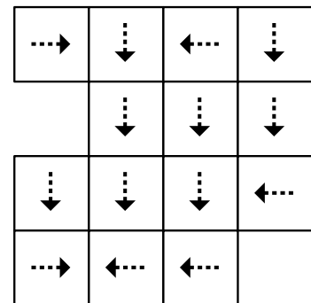
Figure 63 An optimal policy for the cockroach robot world.
