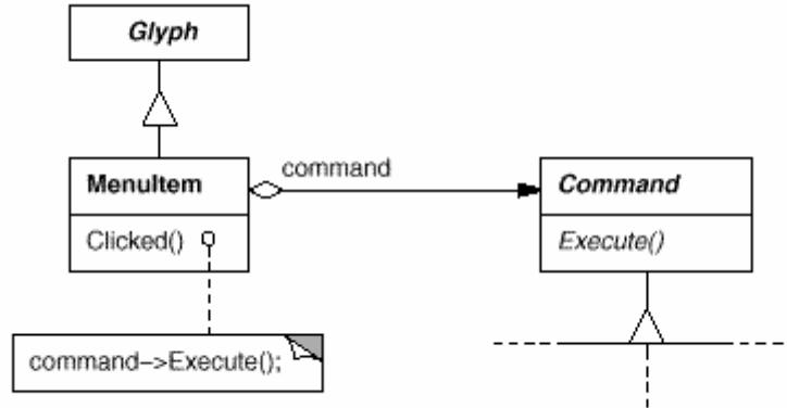
Figure 2.12: MenuItem-Command relationship
