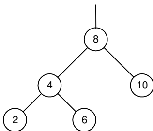
Fig. 4.31. Balanced tree
