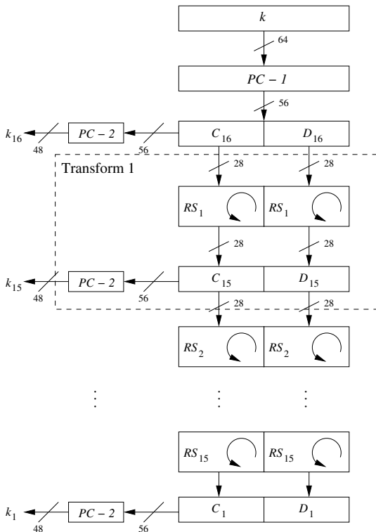
Fig. 3.16 Reversed key schedule for decryption of DES
