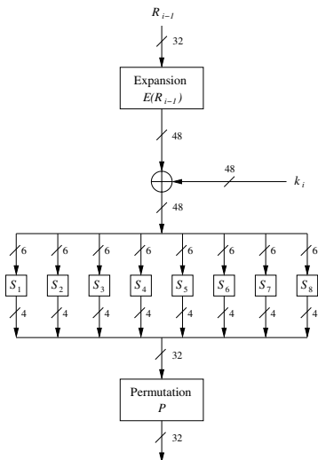
Fig. 3.10 Block diagram of the f -function
