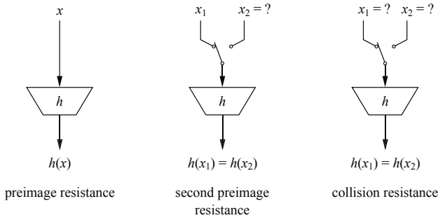
Fig. 11.4 The three security properties of hash functions
