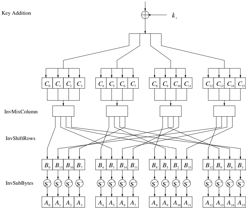
Fig. 4.9 AES decryption round function 1, 2, \dots, n_r - 1
