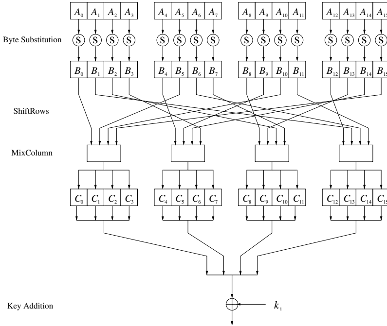
Fig. 4.3 AES round function for rounds 1, 2, \dots, n_r - 1
