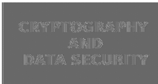
Fig. 5.3 Image and encrypted image using AES with 256-bit key in ECB mode
