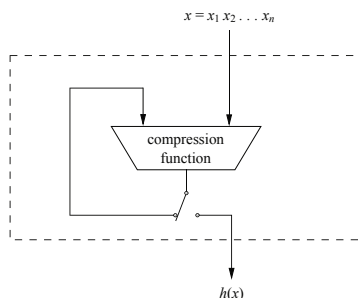
Fig. 11.5 Merkle–Damgård hash function construction
