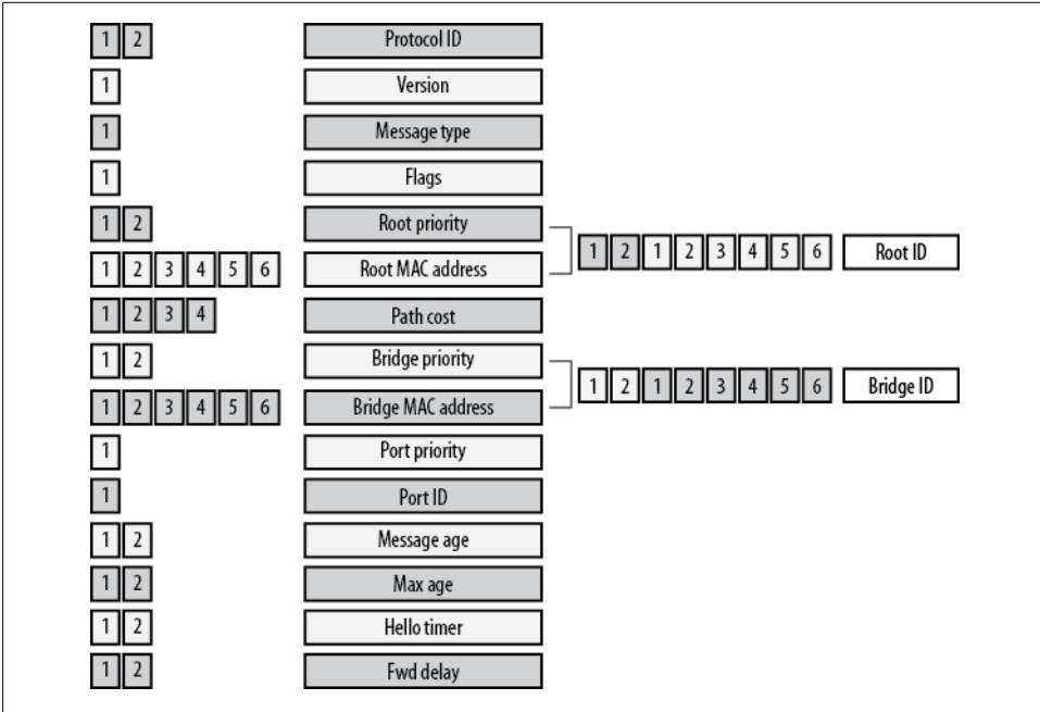
Figure 8-4. BPDUs format
