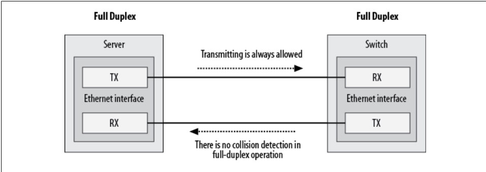
Figure 3-2. Full duplex
