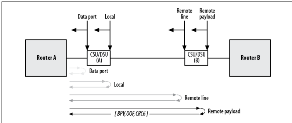
Figure 21-12. Loopback testing progression
