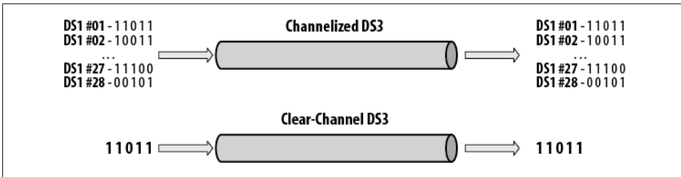
Figure 22-4. Channelized versus clear-channel DS3
