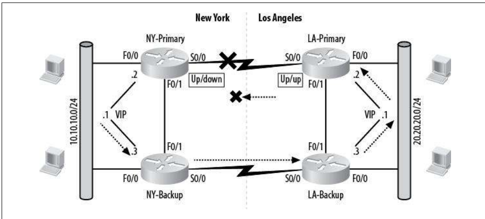
Figure 13-5. HSRP limitations
